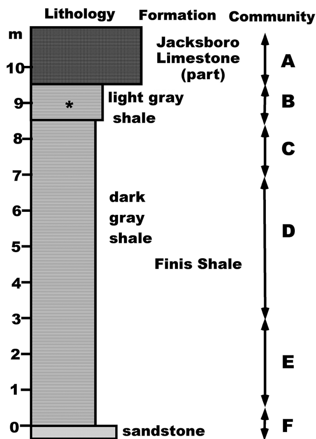
Figure 3. Biotic communities of the Finis Shale and enclosing strata at Jacksboro, Texas (modified from Lobza et al., 1994): A = platy algae; B = high-diversity Lagerstätte; C = Hustedia-Rhipidomella ; D = Crurithyris-Glabrocingulum ; E = Crurithyris-Paraconularia ; F = myalinid; * = source of Willipteria n. gen. specimens.
