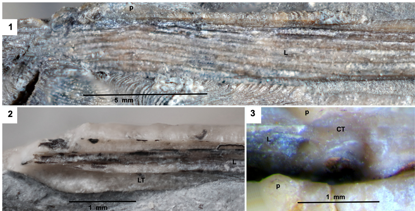
Figure 2. (1–3) Hinge of Willipteria nestelli n. gen. n. sp. (1) Left valve showing small umbo and right valve (behind) showing wavy segment of clinovincular ligament (L) close to beak of the shell; black wedge in lower left corner of photo is an open fracture in shell produced during sediment compaction; P = prodissoconch; paratype, NPL 90424. (2) Small posterior lateral tooth (LT) on left valve of juvenile specimen; paratype, NPL 90434. (3) Cardinal teeth (CT) and narrow ligament (L) on left valve and prodissoconchs (p) of both valves of juvenile specimen; paratype, NPL 90436. All from Finis cycle, Graham Formation, Jacksboro, Texas, USA; Late Pennsylvanian, basal Virgilian (Gzhelian) stage.
