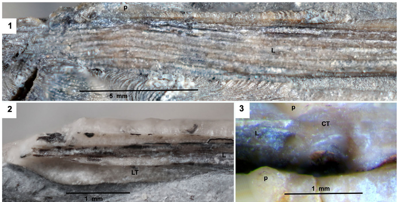
Figure 2. (1–3) Hinge of Willipteria nestelli n. gen. n. sp. (1) Left valve showing small umbo and right valve (behind) showing wavy segment of clinovincular ligament (L) close to beak of the shell; black wedge in lower left corner of photo is an open fracture in shell produced during sediment compaction; P = prodissoconch; paratype, NPL 90424. (2) Small posterior lateral tooth (LT) on left valve of juvenile specimen; paratype, NPL 90434. (3) Cardinal teeth (CT) and narrow ligament (L) on left valve and prodissoconchs (p) of both valves of juvenile specimen; paratype, NPL 90436. All from Finis cycle, Graham Formation, Jacksboro, Texas, USA; Late Pennsylvanian, basal Virgilian (Gzhelian) stage.
