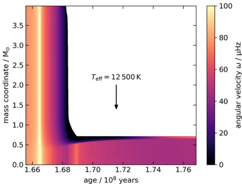
Figure 1. Kippenhahn-type diagram of the mass donor of our fiducial binary model, showing the internal evolution of its rotational frequency (colorbar on the right) after TAMS. The arrow marks the time corresponding to LB-1.
