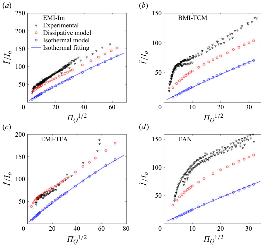
Figure 4. Total current as a function of the dimensionless flow rate for EMI-Im (a), BMI-TCM (b), EMI-TFA (c) and EAN (d). The characteristic scale I_o for each liquid is 2.77 \times 10^{-9} A for EMI-Im, 4.58 \times 10^{-9} A for BMI-TCM, 4.07 \times 10^{-9} A for EMI-TFA and 4.26 \times 10^{-9} A for EAN. We also plot the best fitting function for the combined isothermal data, \tilde{I}/I_o = 2.52 + 2.32\Pi_Q^{1/2} - 0.0049\Pi_Q .
