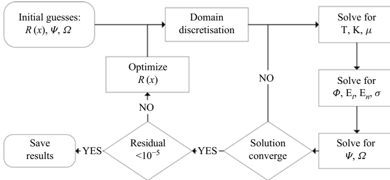
Figure 2. Solution scheme.
