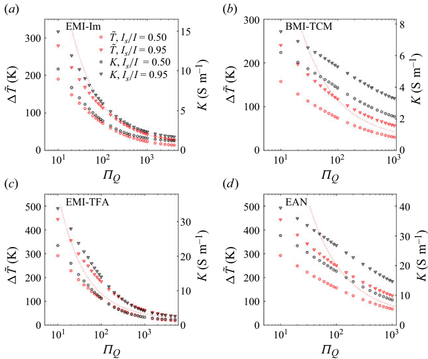
Figure 6. Temperature increase (red) and electrical conductivity (black) at the current cross-over and at I_s/I = 0.95 , for EMI-Im (a), BMI-TCM (b), EMI-TFA (c) and EAN (d). The dashed lines show the regression law for the temperature found by Magnani & Gamero-Castaño (2024), equation (3.3).
