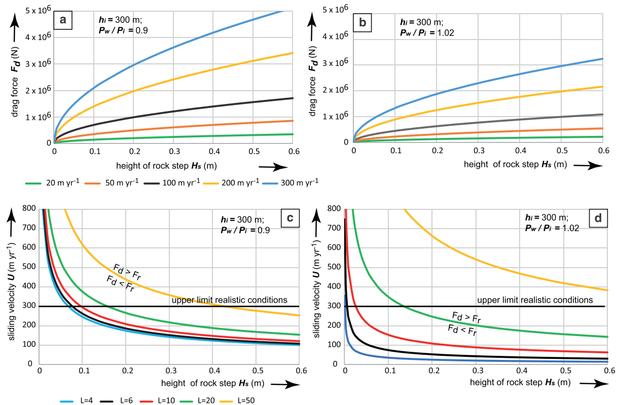
Fig. 10. (a) Drag forces (N) on a flat surface with a rock step, as a function of height of rock step H_s for different ice velocities; Eqn (24). Width and height of blocks are 5 and 2 m; ice thickness = 300 m, P_w/P_i = 0.9 . (b) Same as (a), with P_w/P_i = 1.02 (2% overpressure). (c) Lines of equal drag and resisting forces ( F_d = F_r ) as a function of sliding velocity and height of rock step, for different cumulative length of blocks, P_w/P_i = 0.9 ; Eqn (26). (d) Same as (c), with P_w/P_i = 1.02 (2% overpressure). Figure © Svensk Kärnbränslehantering. Reproduced with permission.
