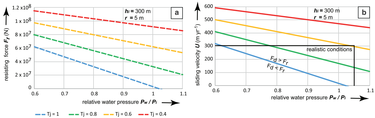
Fig. 8. Effect of limited transmissivity along basal fractures; ice thickness 300 m; hemispherical obstacle with r = 5 . (a) Resisting force in N versus relative water pressure, with transmissivity factor T_j varying between 0.4 and 1; Eqn (16). (b) Lines where drag forces equal resisting forces ( F_d = F_r ) as a function of sliding speed U and relative water pressure P_w/P_i , for hemispherical obstacles with 5 m radius, with transmissivity factor T_j between 0.4 and 1; Eqn (21) with T_j , as per Eqn (16). Above the lines, blocks can move. Box indicates realistic conditions. Figure © Svensk Kärnbränslehantering. Reproduced with permission.
