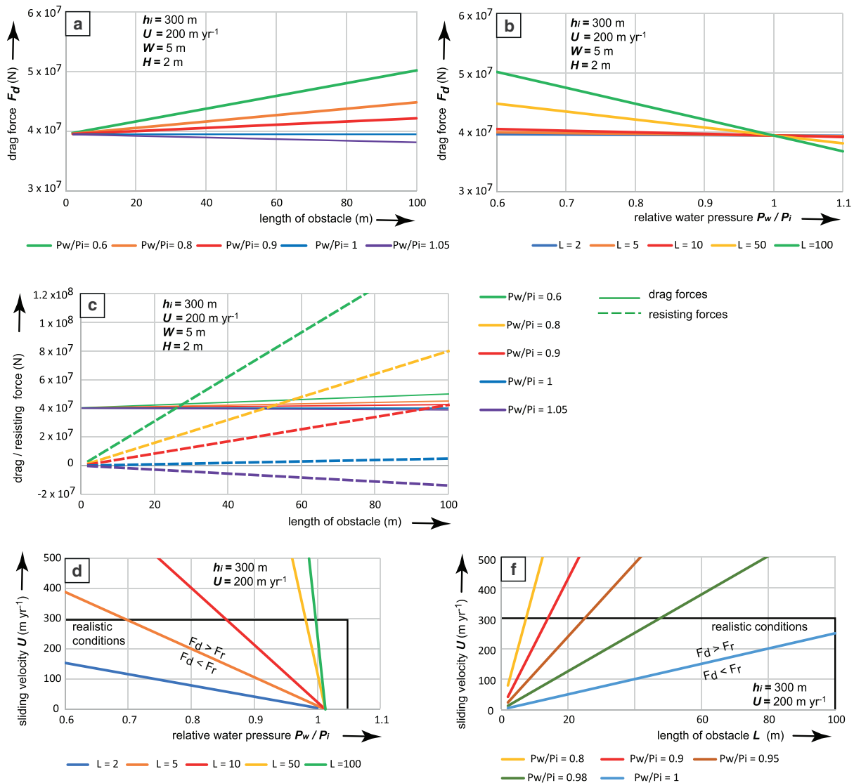
Fig. 9. (a) Drag forces (N) as a function of length of an elongate obstacle, for different relative water pressures; W = 5 , H = 2 m, h_i = 300 m, sliding velocity U = 200 m a ^{-1} ; Eqn (10b). (b) Drag forces as a function of relative water pressure, for obstacles with different lengths; other conditions same as (a); Eqn (10b). (c) Resisting forces (dashed lines; Eqn (15c)) and drag forces (solid lines; Eqn (10b)) as a function of length of a rectangular obstacle ( W = 5 , H = 2 m), for different relative water pressures P_w/P_i ; ice thickness 300 m; ice sliding velocity 200 m a ^{-1} . (d) Lines of equal drag and resisting forces ( F_d = F_r ) as a function of sliding speed U and relative water pressure P_w/P_i , for rectangular obstacles; Eqn (23). Above the lines, blocks can move. Box indicates realistic conditions. (e) Lines of equal drag and resisting forces ( F_d = F_r ) as a function of sliding speed U and obstacle length, for different relative water pressures P_w/P_i (0.8–1.05); Eqn (23). Figure © Svensk Kärnbränslehantering. Reproduced with permission.
