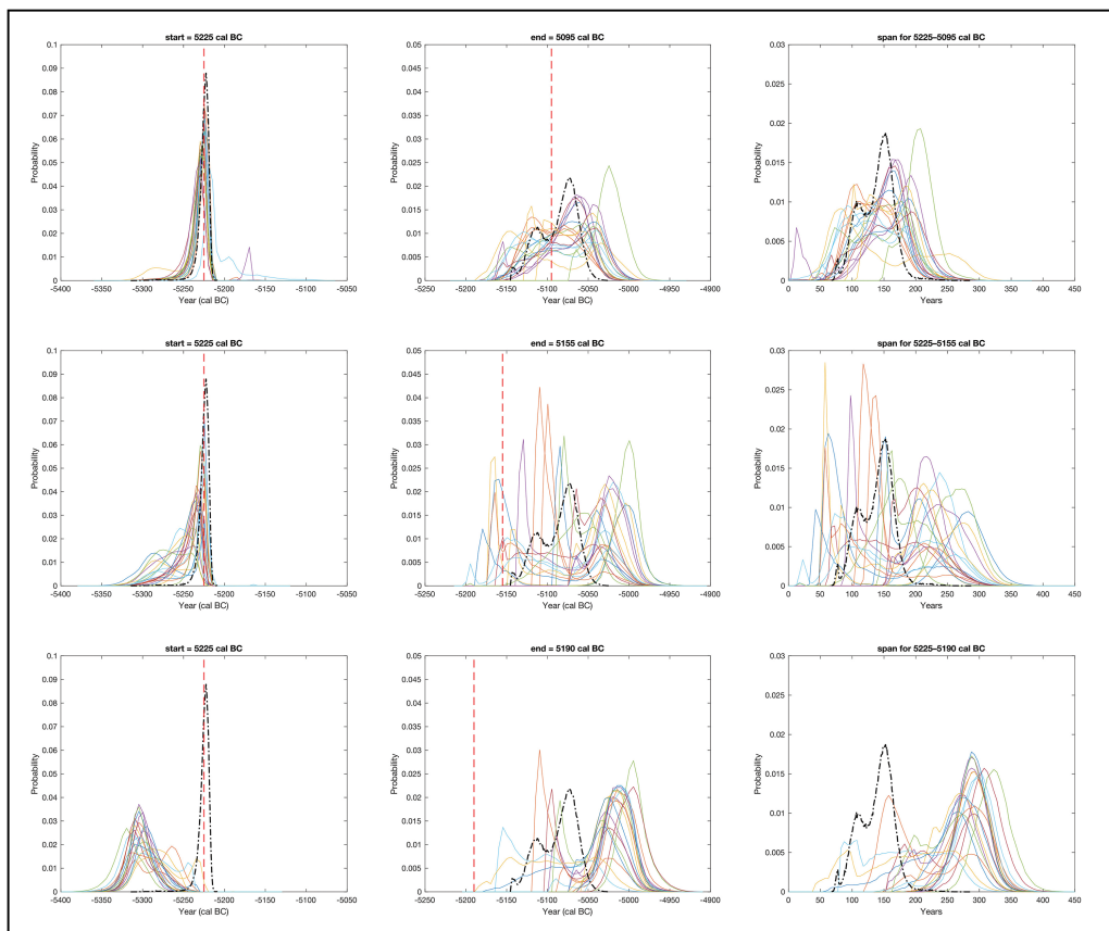
Figure 5. Single bounded-phase Bayesian model of the Schwetzingen cemetery, along with its corresponding simulations. The black dashed line represents the probability based on the model; coloured lines depict the outcomes from 20 different runs of the simulation with 58 dates spaced uniformly between three chronologies: long (top) = 5225–5095 cal BC; short (middle) = 5225–5155 cal BC; and very short (bottom) = 5225–5190 cal BC chronologies (figure by authors).
