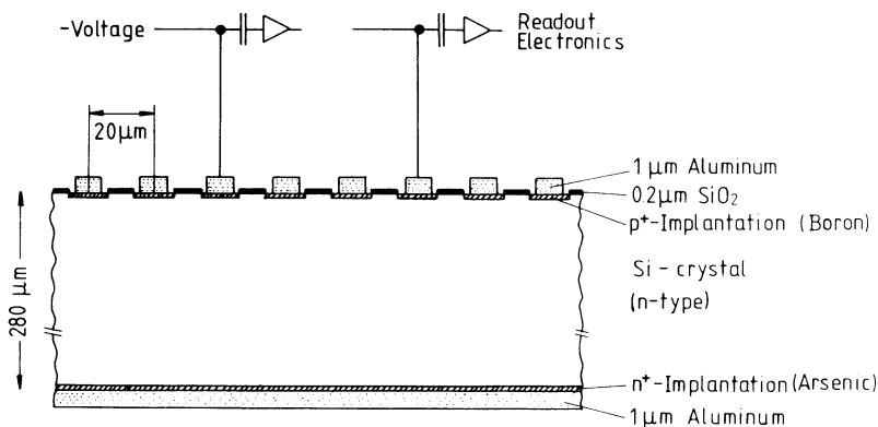
Figure 12.4 Cross section of a silicon microstrip detector. (B. Hyams et al., Nuc. Instr. Meth. 205: 99, 1983.)
