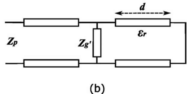
Figure 6. (a) Presented structure for CFRP covered by square patch array resonator and (b) equivalent transmission line model.
