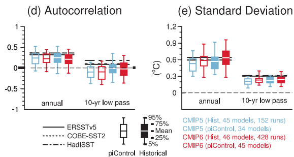
Figure 3.39 | Model evaluation of the Pacific Decadal Variability (PDV). (a, b) Sea surface temperature (SST) anomalies (°C) regressed onto the Tripole Index (TPI; Henley et al., 2015) for 1900–2014 in (a) ERSST version 5 and (b) CMIP6 multi-model ensemble (MME) mean composite obtained by weighting ensemble members by the inverse of the model ensemble size. A 10-year low-pass filter was applied beforehand. Cross marks in (a) represent regions where the anomalies are not significant at the 10% level based on a t-test. Diagonal lines in (b) indicate regions where less than 80% of the runs agree in sign. (c) A Taylor diagram summarizing the representation of the PDV pattern in CMIP5 (each ensemble member is shown as a cross in light blue, and the weighted multi-model mean as a dot in dark blue), CMIP6 (each ensemble member is shown as a cross in red, and the weighted multi-model mean as a dot in orange) and observations over 40°S–60°N and 110°E–70°W. The reference pattern is taken from ERSST version 5 and black dots indicate other observational products: Hadley Centre Sea Ice and Sea Surface Temperature data set version 1 (HadISST version 1) and Centennial in situ Observation-Based Estimates of Sea Surface Temperature version 2 (COBE-SST2). (d) Autocorrelation of unfiltered annual TPI at lag one year and 10-year low-pass filtered TPI at lag 10 years for observations over 1900–2014 (horizontal lines), 115-year chunks of pre-industrial control simulations (open boxes) and individual historical simulations over 1900–2014 (filled boxes) from CMIP5 (blue) and CMIP6 (red). (e) As in (d), but showing standard deviation of the unfiltered and filtered TPI (°C). Boxes and whiskers show weighted multi-model means, interquartile ranges and 5th and 95th percentiles. (f) Time series of the 10-year low-pass filtered TPI (°C) in ERSST version 5, HadISST version 1 and COBE-SST2 observational estimates (black) and CMIP5 and CMIP6 historical simulations. The thick red and light blue lines are the weighted multi-model mean for the historical simulations in CMIP5 and CMIP6, respectively, and the envelopes represent the 5th–95th percentile ranges across ensemble members. The 5–95% confidence interval for the CMIP6 multi-model mean is given in thin dashed lines. Further details on data sources and processing are available in the chapter data table (Table 3.SM.1).
