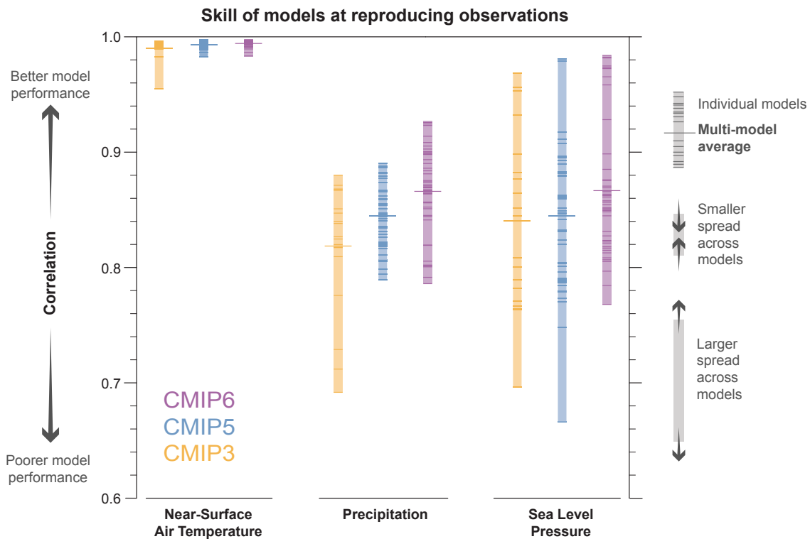
FAQ 3.3, Figure 1 | Pattern correlations between models and observations of three different variables: surface air temperature, precipitation and sea level pressure. Results are shown for the three most recent generations of models, from the Coupled Model Intercomparison Project (CMIP): CMIP3 (orange), CMIP5 (blue) and CMIP6 (purple). Individual model results are shown as short lines, along with the corresponding ensemble average (long line). For the correlations the yearly averages of the models are compared with the reference observations for the period 1980–1999, with 1 representing perfect similarity between the models and observations. CMIP3 simulations performed in 2004–2008 were assessed in the IPCC Fourth Assessment, CMIP5 simulations performed in 2011–2013 were assessed in the IPCC Fifth Assessment, and CMIP6 simulations performed in 2018–2021 are assessed in this Report.
