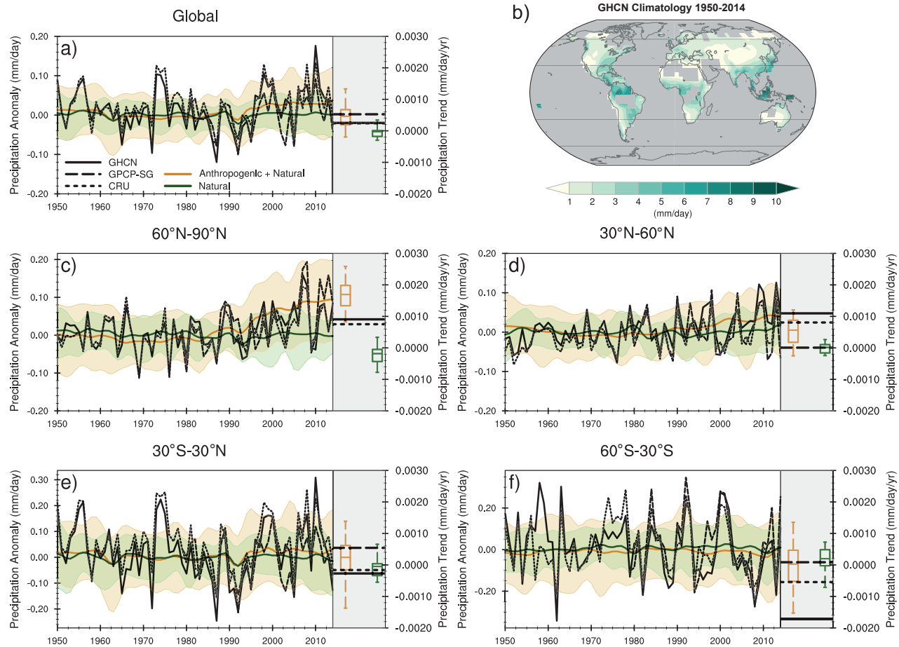
Figure 3.15 | Observed and simulated time series of anomalies in zonal average annual mean precipitation. (a), (c–f) Evolution of global and zonal average annual mean precipitation ( \text{mm day}^{-1} ) over areas of land where there are observations, expressed relative to the base period of 1961–1990, simulated by CMIP6 models (one ensemble member per model) forced with both anthropogenic and natural forcings (brown) and natural forcings only (green). Multi-model means are shown in thick solid lines and shading shows the 5–95% confidence interval of the individual model simulations. The data is smoothed using a low pass filter. Observations from three different datasets are included: gridded values derived from Global Historical Climatology Network (GHCN version 2) station data, updated from Zhang et al. (2007), data from the Global Precipitation Climatology Product (GPCP L3 version 2.3, Adler et al. (2003)) and from the Climate Research Unit (CRU TS4.02, Harris et al. (2014)). Also plotted are boxplots showing interquartile and 5–95% ranges of simulated trends over the period for simulations forced with both anthropogenic and natural forcings (brown) and natural forcings only (blue). Observed trends for each observational product are shown as horizontal lines. Panel (b) shows annual mean precipitation rate ( \text{mm day}^{-1} ) of GHCN version 2 for the years 1950–2014 over land areas used to compute the plots. Further details on data sources and processing are available in the chapter data table (Table 3.SM.1).
