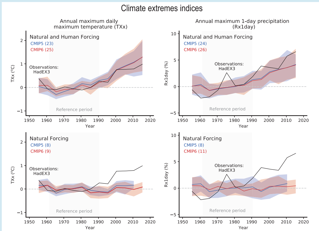
Cross-Chapter Box 3.2, Figure 1 | Comparison of observed and simulated changes in global mean temperature and precipitation extremes. Time series of globally averaged five-year mean anomalies of the annual maximum daily maximum temperature (TXx in °C) and annual maximum 1-day precipitation (Rx1day as standardized probability index in %) between 1953 and 2017 from the HadEX3 observations and the CMIP5 and CMIP6 multi-model ensembles with natural and human forcing ( top ) and natural forcing only ( bottom ). For CMIP5, historical simulations for 1953–2005 are combined with corresponding RCP4.5 scenario runs for 2006–2017. For CMIP6, historical simulations for 1953–2014 are combined with SSP2-4.5 scenario simulations for 2015–2017. Numbers in brackets represent the number of models used. The time-fixed observational mask has been applied to model data throughout the whole period. Grid cells with more than 70% of data available between 1953 and 2017 plus data for at least three years between 2013 and 2017 are used. Coloured lines indicate multi-model means, while shading represents 5th–95th percentile ranges, based on all available ensemble members with equal weight given to each model (Section 3.2). Anomalies are relative to 1961–1990 means. Figure is updated from Seong et al. (2021), their Figure 3 and Paik et al. (2020b), their Figure 3. Further details on data sources and processing are available in the chapter data table (Table 3.SM.1).
