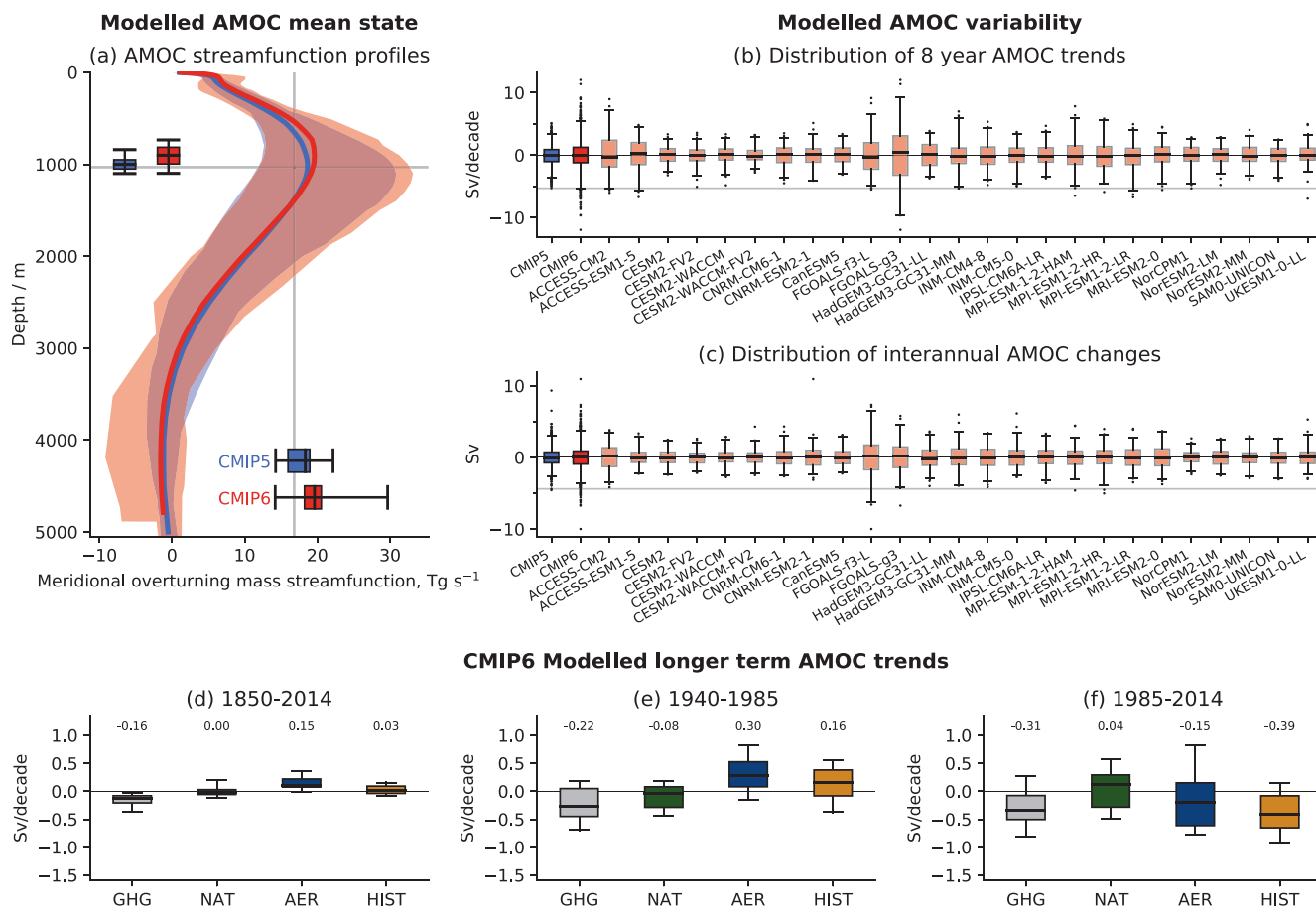
Figure 3.30 | Observed and CMIP6 simulated AMOC mean state, variability and long-term trends. (a) AMOC meridional stream function profiles at 26.5^{\circ}N from the historical CMIP5 (1860–2004) and CMIP6 (1860–2014) simulations compared with the mean maximum overturning depth (horizontal grey line) and magnitude (vertical grey line) from the RAPID observations (2004–2018). The distributions of model ranges of AMOC maximum magnitude and depth are respectively displayed near the x- and y-axis. (b) Distributions of overlapping eight-year AMOC trends from individual CMIP6 historical simulations (pink box plots) are plotted along with the combined distributions of all available CMIP5 (blue boxplot) and CMIP6 (red boxplot) models. For reference, the observed eight-year trend calculated between 2004 and 2012 is also shown as a horizontal grey line (following Roberts et al., 2014). (c) Distributions of interannual AMOC variability from individual CMIP6 model historical simulations, along with the combined distributions of all available CMIP5 and CMIP6 models. Interannual variability in models and observations is estimated as annual mean (April–March) differences, and the horizontal grey line is the observed value for 2009/2010 minus 2008/2009 (following Roberts et al., 2014). (d–f) Distributions of linear AMOC trends calculated over various time periods (see panel titles) in CMIP6 simulations forced with: greenhouse gas forcing only (GHG), natural forcing only (NAT), anthropogenic aerosol forcing only (AER) and all forcing combined (Historical; HIST). (a–f) Boxes indicate the 25th to 75th percentile range, whiskers indicate 1st and 99th percentiles in (a–c) and 5th and 95th percentile in (d–f), and dots indicate outliers, while the horizontal black line is the multi-model mean trend. In (d–f) the multi-model mean trend is also written above each distribution. The multi-model distributions in (a–c) were produced with one historical ensemble member per model for which the AMOC variable was available (listed), while those in (d–f) were produced with the detection and attribution simulation datasets utilized by Menary et al. (2020). Further details on data sources and processing are available in the chapter data table (Table 3.SM.1).
