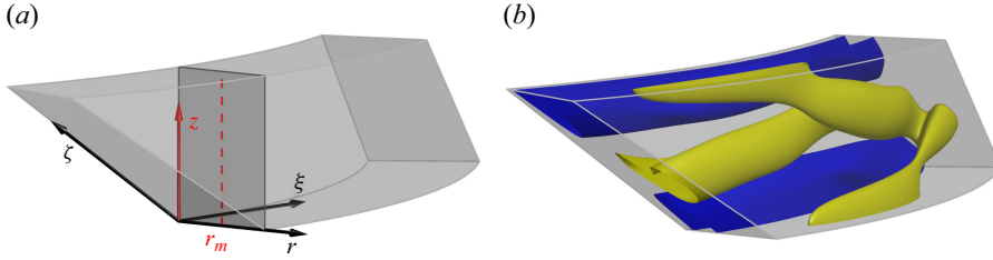
Figure 2. (a) Annular-parallelogram computational domain defined by the coordinates of (2.7) with wavenumbers (n_1, k_1, n_2, k_2) = (10, 2, 0, 4.5) and \eta = 0.883 , adopted from W22. The axial line probe (red dashed vertical line) used in the production of space–time diagrams is located at mid gap r_m = (r_i + r_o)/2 \approx 8.047 . (b) Three-dimensional flow structure of DRW solution for (R_i, R_o) = (450, -1200) . Positive (yellow, u_\theta = 250 ) and negative (blue, u_\theta = -100 ) isosurfaces of perturbation azimuthal velocity.
