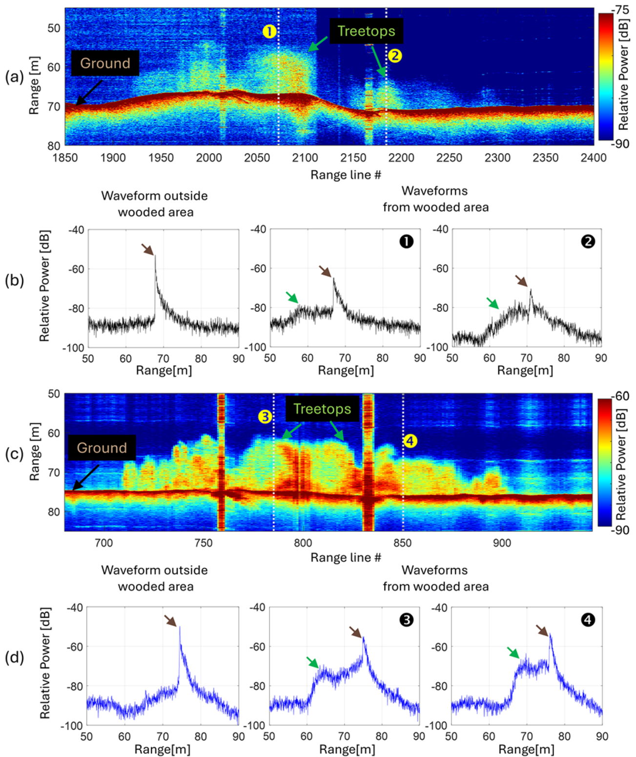
Figure 11. Zoomed view of the 2.6–7 GHz echogram over the woodland without vehicle's altitude correction (a) and representative waveforms (b). Zoomed view of the 12–18 GHz echogram over the woodland without vehicle's altitude correction (c) and representative waveforms (d). For (b) and (d), the left insets correspond to surface returns over grass-covered ground outside the forested section. The mid and right insets correspond to waveforms collected over the treed area at the locations marked as (1), (2) in the 2.6–7 GHz echogram and as (3), (4) in the 12–18 GHz image. The green arrows point to the response from the tree canopies. The brown arrows point to the return from the ground. Range is in meters assuming free space propagation.
