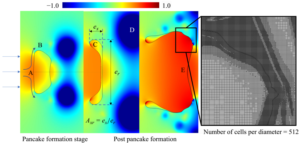
Figure 4. Non-dimensional pressure field P/(\rho_o V_0^2) renders for a drop undergoing backward bag fragmentation. Labelled A–E in the figure are the points of interest in a deforming drop and relate to the following features: the upstream pole/core of the drop (A); the periphery of the drop (B); the rim of the drop, which in general has a higher local inertia compared with its centre (C); the downstream low pressure circulation zone, which can affect the motion of its rim if it is attached to the drop surface (unlike in the figure) (D); and the inflated bag, which inflates because of its low inertia and, hence, higher accelerations (E).
