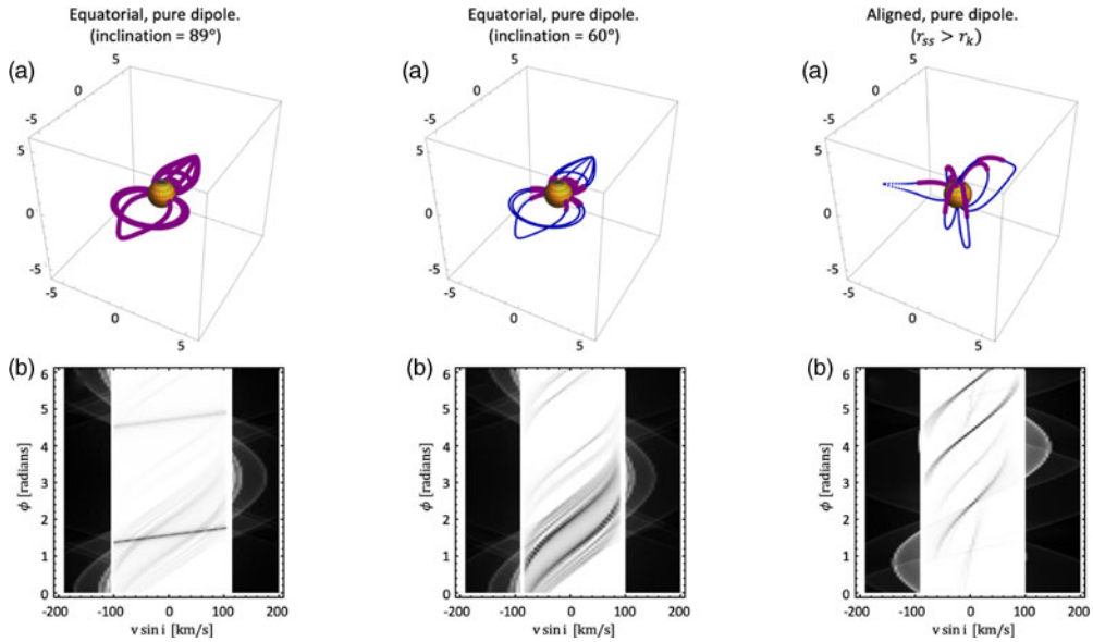
Figure 1. Example magnetic field lines (blue) and visible sections (purple) and below, the associated H \alpha trails.
