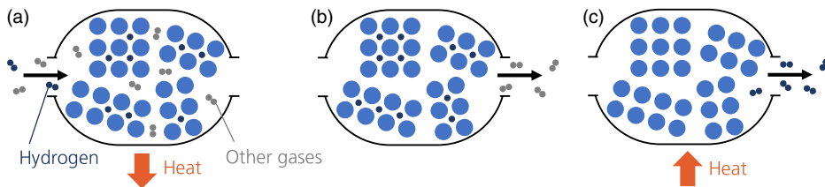
Figure 9. Working principle of hydrogen purification by MHs according to Ref. (6): (a) filling with impure hydrogen and absorption, (b) flushing of admixtures and (c) desorption of pure hydrogen.
