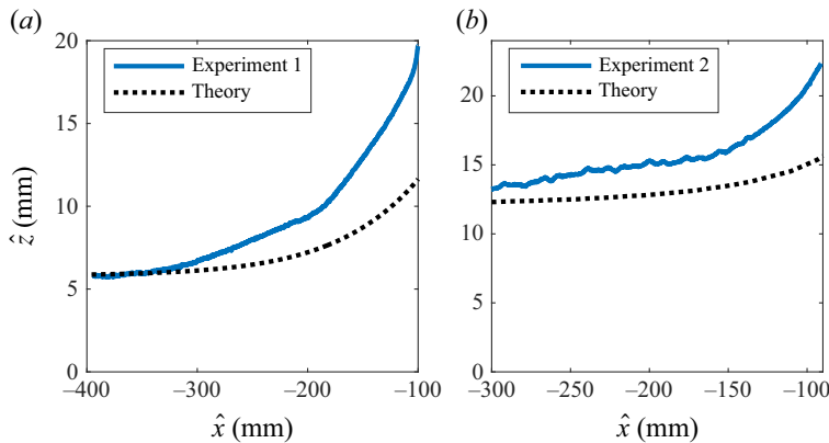
Figure 13. Fluid thickness along the centreline measured in (a) experiment 1 and (b) experiment 2 after 60 minutes, and the final arrested state predicted by (3.10a)–(3.15).
