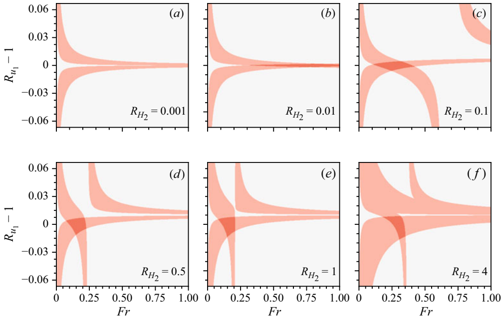
Figure 9. Illustrative computations of the eigenvalues of \hat{\mathbf{B}}_{red} for the model of Pudasaini & Mergili (2019), with R_{H_1} = 1 and R_{u_2} = 1.01 . In regions shaded pink, the model possesses a single pair of complex eigenvalues, while red shading covers areas where two complex pairs were found. Elsewhere, all eigenvalues are real. The parameters for these computations are given in Appendix C.
