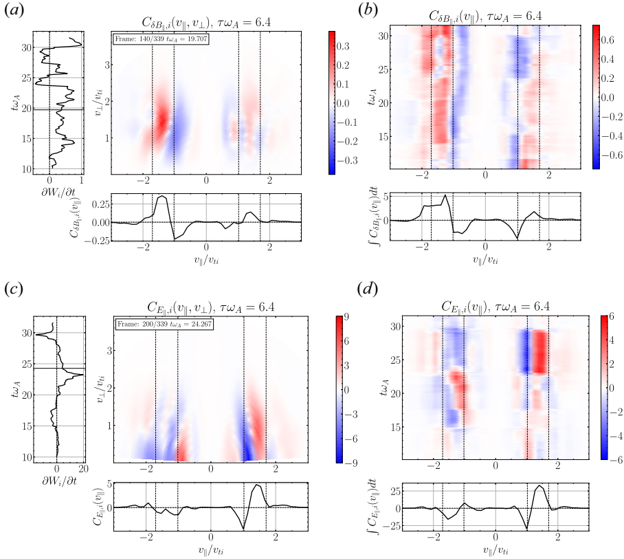
FIGURE 10. Velocity-space signatures of TTD ( a,b ) at probe 13 ( \pi\rho_i, 7\pi\rho_i, 0 ) and LD ( c,d ) at probe 24 ( 4\pi\rho_i, 4\pi\rho_i, 0.875\pi a_0 ) in AstroGK turbulence simulation with 0.25 \leq k_{\perp}\rho_i \leq 7.75 , T_i/T_e = 1 , and \beta_i = 1 . The correlation interval is set as \tau\omega_A = 6.4 . ( a,c ) Gyrotropic plane ( v_{\parallel}, v_{\perp} ) signatures, following the layout format of panels in figure 4. ( b,d ) Timestack plots of the v_{\perp} -integrated reduced correlation; the main panel here shows the reduced correlation on (v_{\parallel}, t) grids, and the lower panel shows the time-integrated reduced correlation. Four vertical dashed lines at v_{\parallel}/v_{ti} = \pm 1.020 and v_{\parallel}/v_{ti} = \pm 1.704 indicate the resonant parallel phase velocity ranges where significant ion damping occurs.
