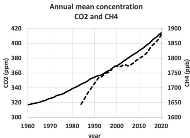
Figure 1.1 Annual mean concentration of carbon dioxide (CO 2 , solid line; in parts per million, ppm) and of methane (CH 4 , dashed line; in parts per billion, ppb), measured at the Mauna Loa Observatory. Source: Carbon dioxide data provided by Dr Pieter Tans, NOAA Global Monitoring Laboratory, Boulder, USA ( gml.noaa.gov/ccgg/trends/ ) and Dr Ralph Keeling, Scripps Institution of Oceanography ( scrippsco2.ucsd.edu/ ). Methane data provided by Ed Dlugokencky, NOAA Global Monitoring Laboratory, Boulder, USA ( gml.noaa.gov/ccgg/trends_ch4 ).
