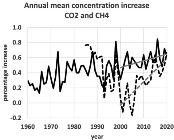
Figure 1.2 Annual percentage increase in the concentration of carbon dioxide ( \text{CO}_2 , solid line) and of methane ( \text{CH}_4 , dashed line), computed from the Mauna Loa Observatory data shown in Figure 1.1. The two lines show the best linear-fit straight lines that fit the data between 2000 and 2020. Source: Data provided by NOAA Global Monitoring Laboratory, Boulder, USA ( https://gml.noaa.gov ).
