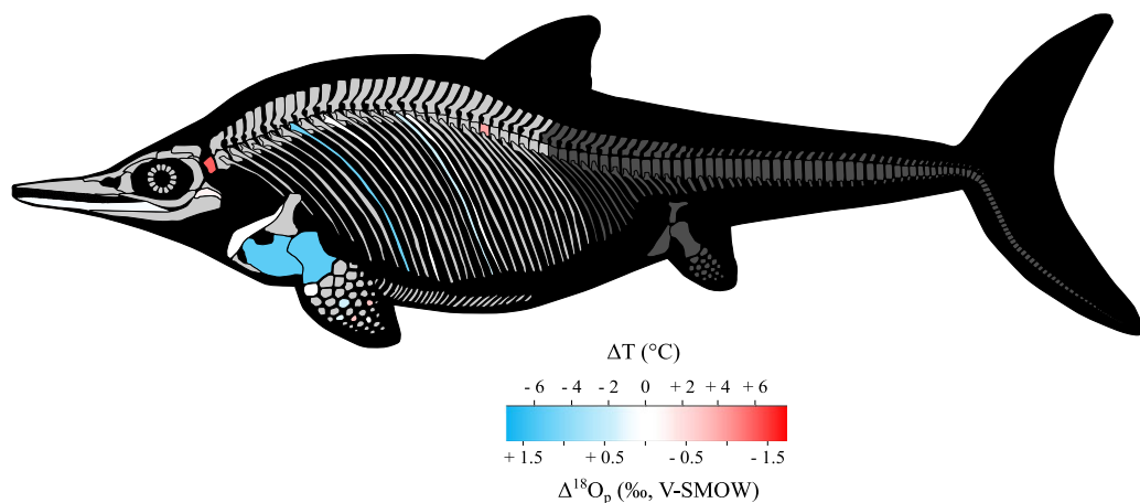
Figure 1. Regional heterothermies in ichthyosaurs. Phosphate oxygen isotope and temperature variability within the skeleton from A , the specimen of Ichthyosauria indet., B , the specimen of Palvennia hoybergeri (PMO 222.669), and C , the specimen of Keilhauia sp. (PMO 222.667). Color in bones corresponds to the \delta^{18}\text{O}_p difference between bone and the midrange value, (\delta^{18}\text{O}_{p-\max} + \delta^{18}\text{O}_{p-\min})/2 , of the skeleton. For paired skeletal elements, the mean value is illustrated. Available skeletal elements are shown in light gray, while unavailable elements and skeletal elements with potentially altered \delta^{18}\text{O}_p values are shown in dark gray. Skeletal elements (e.g., “limb bones”; Supplementary Table 1 ) with precise location unknown are not illustrated, while the locations of vertebrae, ribs, and phalanges that have not been found in articulation have been established arbitrarily. The representation of the organisms is not to scale.
