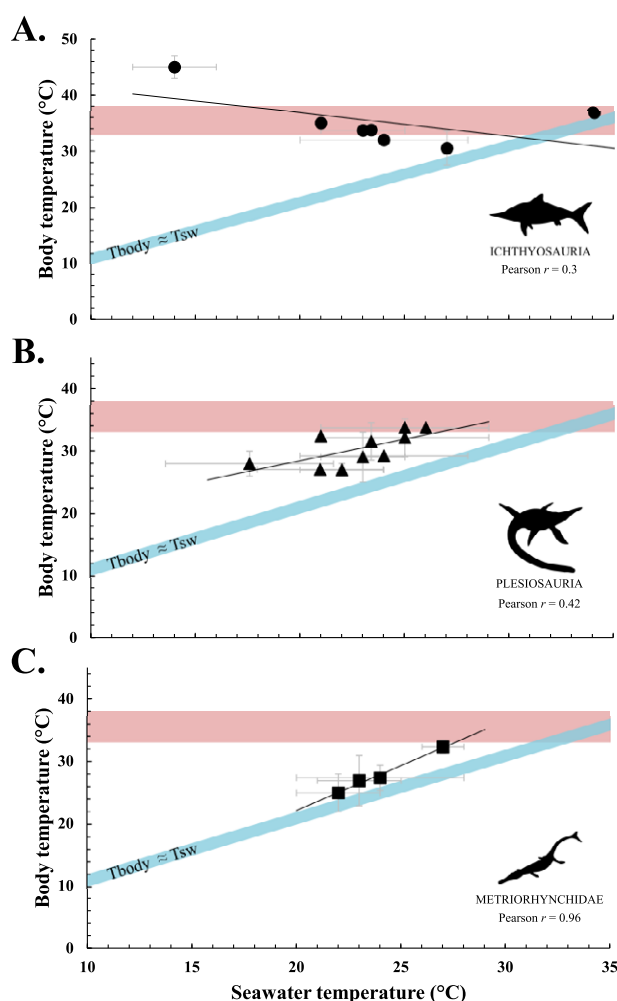
Figure 8. Body temperature estimates of Ichthyosauria (A), Plesiosauria (B), and Metriorhynchidae (C) from tooth enamel \delta^{18}\text{O}_\text{p} values (new data in Supplementary Table 1 and published data in Supplementary Table 2) reported against environmental seawater temperature of their living environments. The body temperature range of extant homeothermic endotherm Cetacea is illustrated in red (Morrison 1962; Hampton et al. 1971; Yeates and Houser 2008), while the body temperature range shown in blue corresponds to the temperature range of a strictly ectothermic poikilothermic model organism whose body temperature is equal to the environmental temperature +2^\circ\text{C} . Body and environmental temperatures were calculated using the equation of Lécuyer et al. (2013) and considering the latitudinal gradient of \delta^{18}\text{O}_\text{sw} values of Alberti et al. (2020) and an ^{18}\text{O} -enrichment of body water relative to environmental water of +0.8 \pm 0.9\text{‰} for Mesozoic marine reptiles (Séon et al. 2023). Silhouettes were made by Gareth Monger for Ichthyosauria and Metriorhynchidae and T. Michael Keesey for Plesiosauria. Images downloaded from PhyloPic and used under a CCBY 3.0 license: https://creativecommons.org/licenses/by/3.0 .
