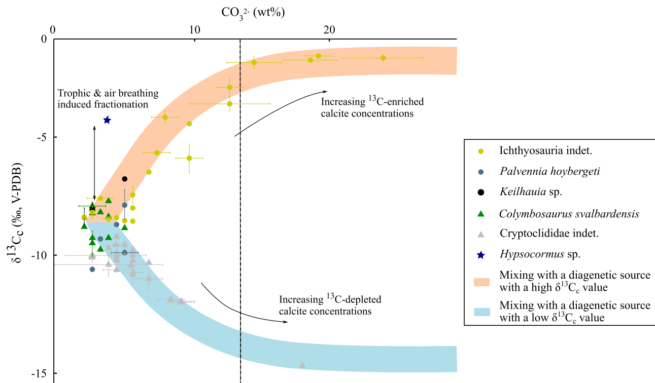
Figure 9. The \delta^{13}\text{C}_c values (‰, VPDB) of bone elements and teeth in ichthyosaurs and plesiosaurs as a function of carbonate content (wt%). The values corresponding to the Hypocormus sp. tooth found in the same stratigraphic layer as the Ichthyosauria indet. specimen are also plotted. The dotted line marks the boundary between mineralized elements with a carbonate content greater than or less than +13.4%.
