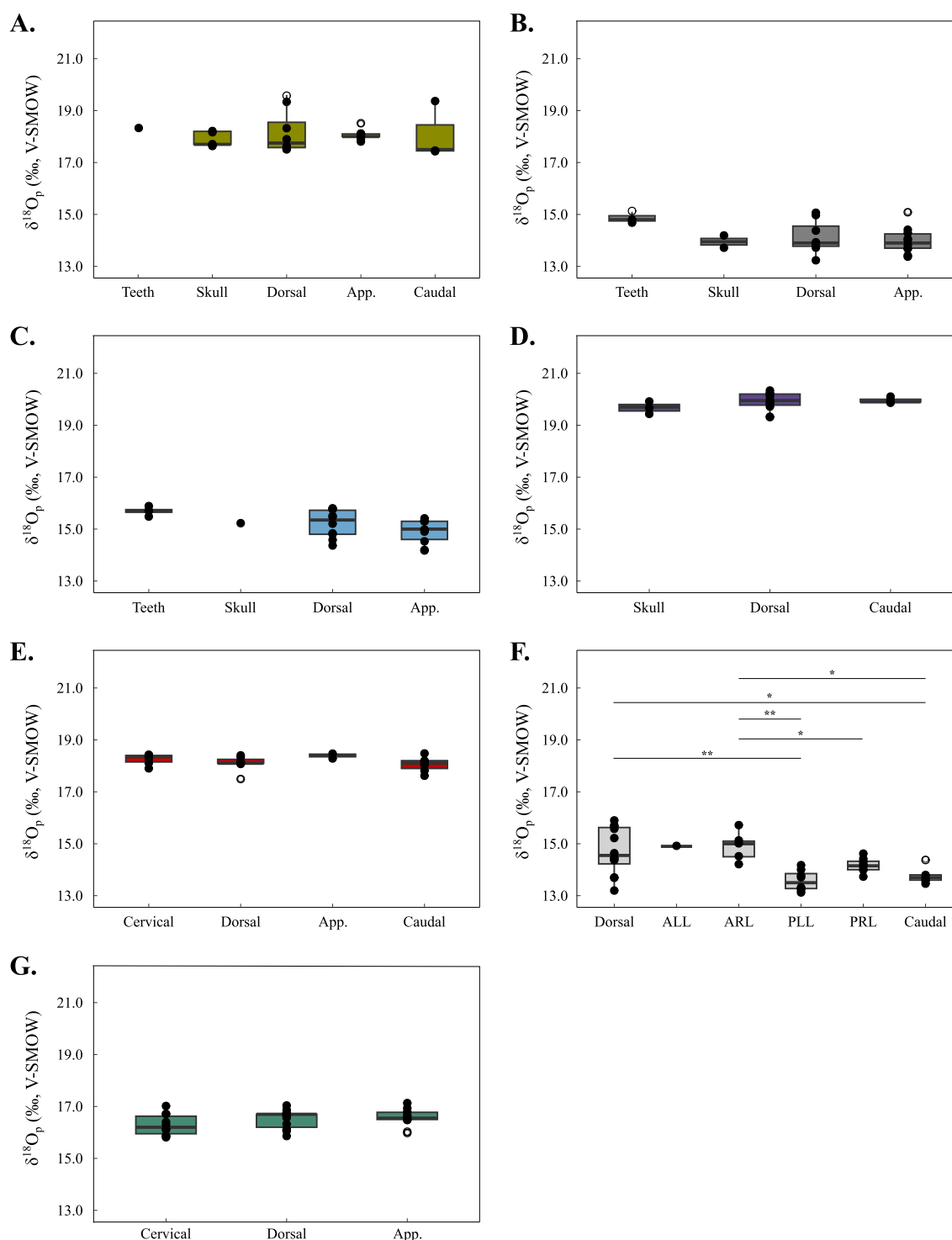
Figure 4. Box plots showing the \delta^{18}\text{O}_p value distribution of bones sets for the specimens of Ichthyosauria ( A , Ichthyosauria indet.; B , Keilhauia sp.; C , Palvennia hoybergeti ), Metriorhynchus aff. supercilius ( D ) and Plesiosauria ( E , Elasmosauridae indet.; F , Colymbosaurus svalbardensis ; and G , Cryptoclididae indet.). Asterisks indicate the significance of the observed differences between pair of groups: * p -value < 0.05; ** p -value < 0.01; *** p -value < 0.001. Outliers are plotted as white circles. The horizontal bars in the boxes correspond to the medians and the whiskers to the minimum and maximum values. The average analytical error for each bone analyzed is on the order of 0.3‰. Abbreviations: App., Appendicular region; ALL, anterior left limb; ARL, anterior right limb; PLL, posterior left limb; PRL, posterior right limb.
