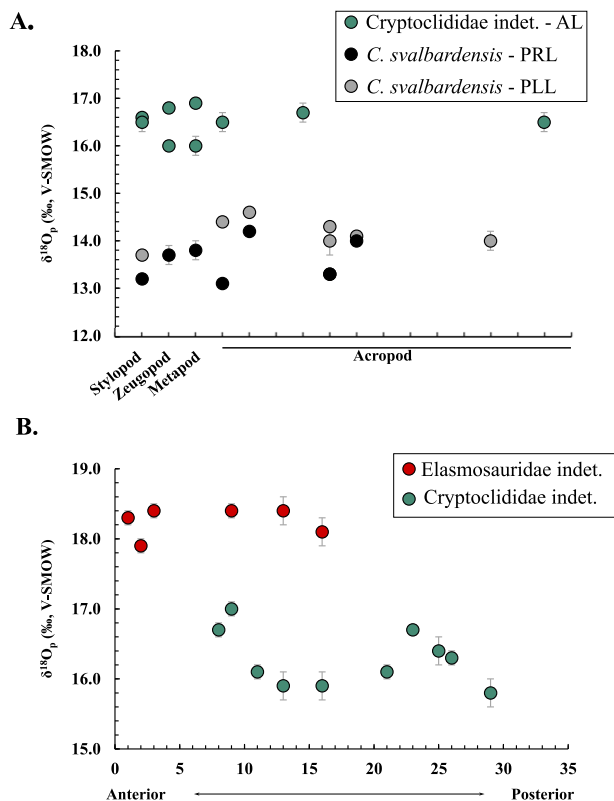
Figure 5. A. \delta^{18}\text{O}_p values (‰, V-SMOW) according to bone position within the limb for the specimen of Cryptoclididae indet. and the specimen of Colymbosaurus svalbardensis . Stylopod set corresponds to the femur or the humerus, Zeugopod set to radius and ulna or tibia and fibula, Metapod set to metacarpals or metatarsals, and Acropod set to phalanges. Abbreviations: AL, Anterior limb indet.; PRL, posterior right limb; PLL, posterior left limb. B. \delta^{18}\text{O}_p values (‰, V-SMOW) according to position of the vertebra within the cervical region for the specimen of Elasmosauridae indet. and the specimen of Cryptoclididae indet.
