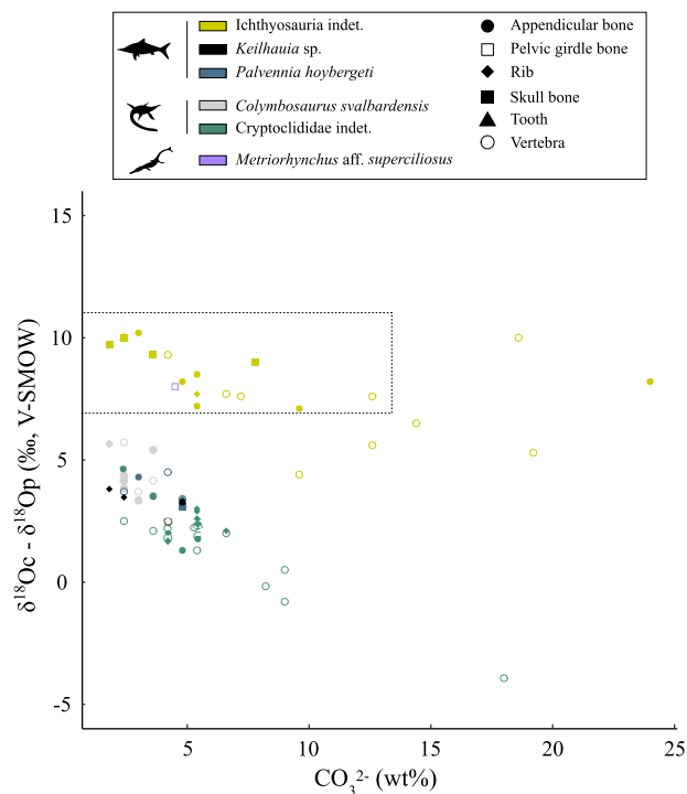
Figure 6. The \delta^{18}\text{O}_c - \delta^{18}\text{O}_p differences between teeth and bone types plotted against carbonate content (wt%) of bioapatite. The dashed rectangle zone corresponds to the combination of parameters that would indicate a potential biological preservation of the oxygen isotope composition of the bioapatite of teeth and bones. Silhouettes were made by Gareth Monger for Ichthyosauria and Metriorhynchidae and T. Michael Keesey for Plesiosaurs. Images downloaded from PhyloPic and used under a CCBY 3.0 license: https://creativecommons.org/licenses/by/3.0 .
