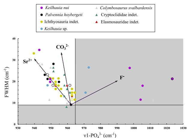
Figure 7. The \nu_1(\text{PO}_4^{3-}) stretching band position and full width at half maximum (FWHM) measured for Ichthyosauria and Plesiosaurs bones and teeth (Supplementary Table 3). Empty symbols represent enamel samples, while solid symbols represent bone samples. The gray zone corresponds to the combination of parameters that would indicate a mineralogical alteration of the bioapatite of teeth and bones. The black arrows indicate the evolution of the position of the \nu_1(\text{PO}_4^{3-}) stretching band position and the FWHM depending on the type of ionic substitution within the bioapatite (Thomas et al. 2011).
