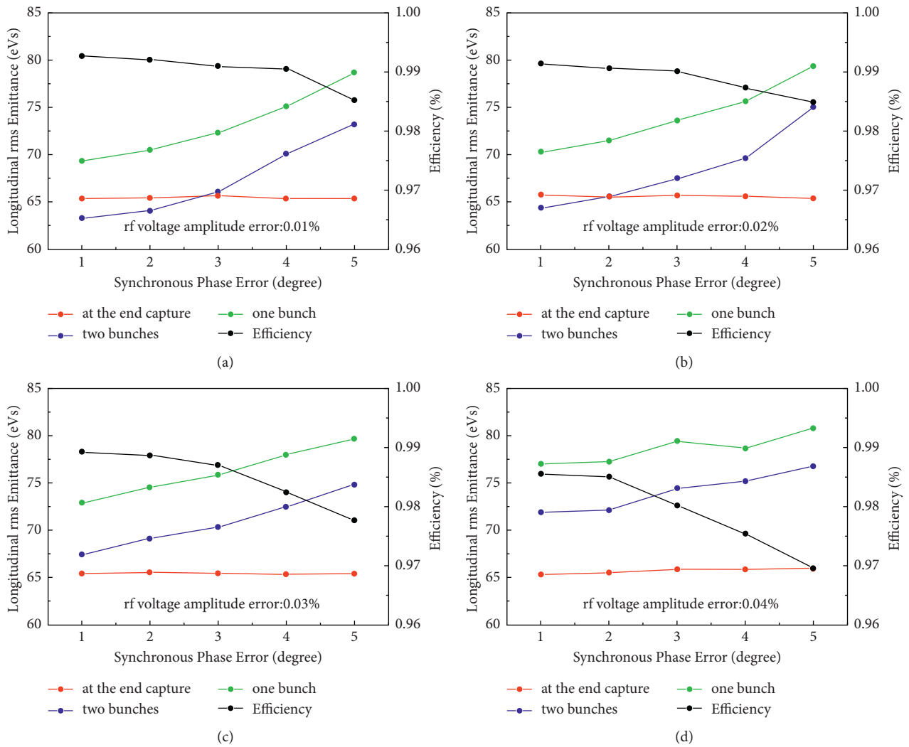
FIGURE 9: \epsilon_{rms} and efficiency vs. RF field errors in phase ( \Delta\phi=1^\circ, 2^\circ, 3^\circ, 4^\circ , and 5^\circ ) and in amplitude ( \Delta V/V ): (a) \Delta V/V = 0.01\% ; (b) \Delta V/V = 0.02\% ; (c) \Delta V/V = 0.03\% ; (d) \Delta V/V = 0.04\% .
