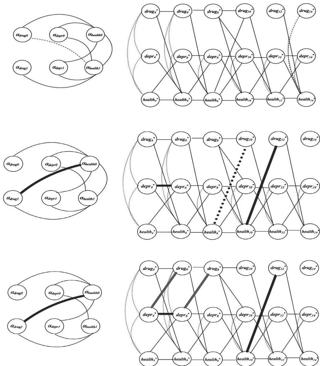
Figure 1. Path diagram depicting the cross-lagged and autoregressive component (right) and multivariate growth part (left) of alternative autoregressive latent trajectory model specifications for illegal drug use ( drug ), depressive symptoms ( depr ), and general health status ( health ). The top panel is based on the standard ( \theta ) parameterization of the auxiliary model linking observed variables to the underlying continuous ones, as adopted by Mplus 8.6 and lavaan 0.6-16. Dashed lines indicate statistically significant effects ( p – value < 0.05) only under this specification. The middle panel showcases an alternative parameterization proposed by Muthén and Asparouhov (2002). Paths in dark gray signify significance under the alternative parameterizations but not under the standard one. The bottom panel employs the parameterization introduced by Jöreskog (2001). Light gray paths indicate a significant pattern under this specification but not in the others.
