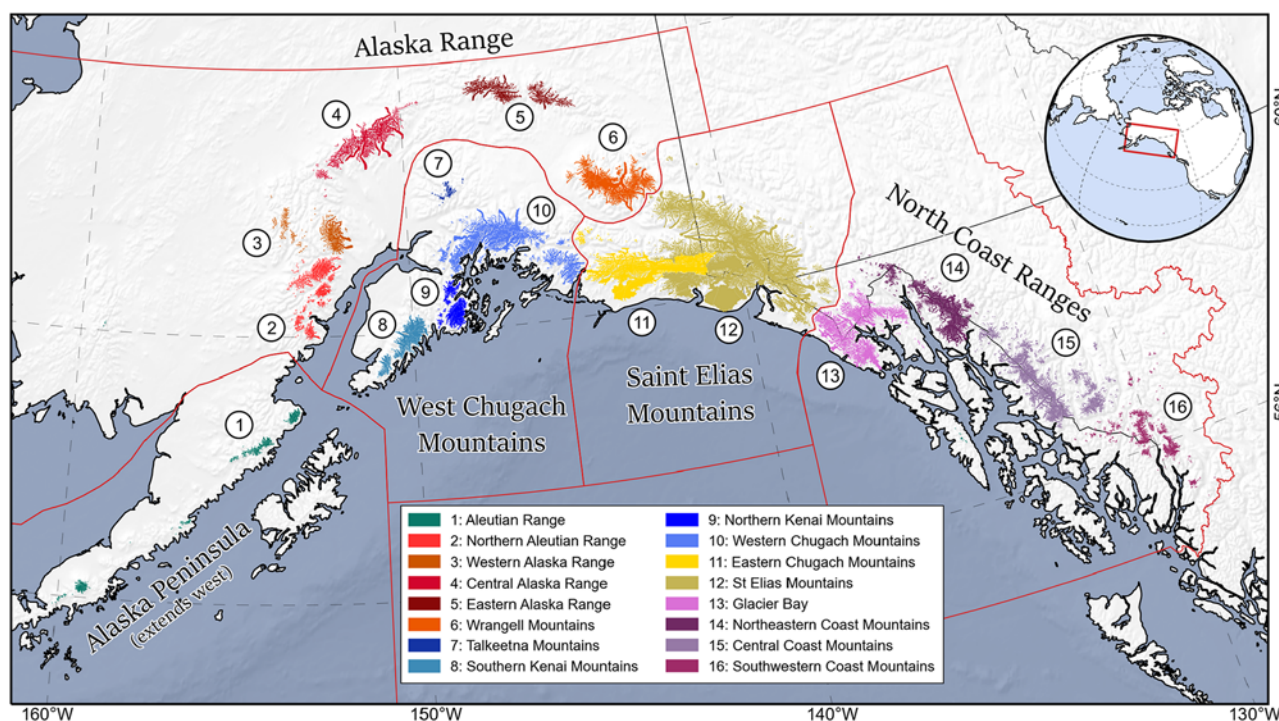
Figure 1. The study area in Alaska and northwest Canada. Glaciers included in the study are mapped, with colors corresponding to their O3Region. The inset legend indicates the color, name and labeled number of each O3Region. Red outlines and corresponding names indicate the O2Regions defined by the RGI (RGI Consortium, 2017). Inset globe and rectangle show the global context of the area. This map and all other figures are presented in the Alaska Albers equal-area projection (EPSG:3338).
