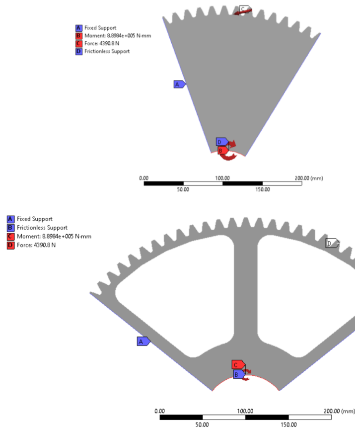
Figure 2. Partitions used for calculation and boundary conditions; referent gear (top) and reduced-mass gears (bottom)
