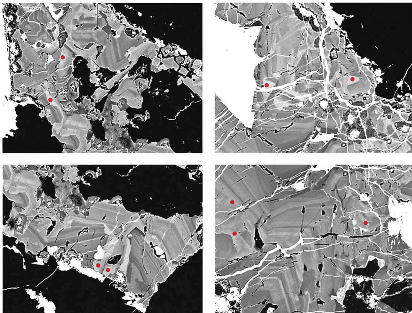
Figure 1. Back-scattered electron images of the chemically zoned grains of Bi-rich tennantite-(Zn) from the Geister vein, Jáchymov, Czech Republic, with zones and domains of annivite-(Zn) marked by red points; white is bismite and other supergene Bi and U minerals. Field of view of all images is 265 \mu\text{m} (sample P1N38896, National Museum Prague, image reproduced from Velebil and Sejkora, 2018).
