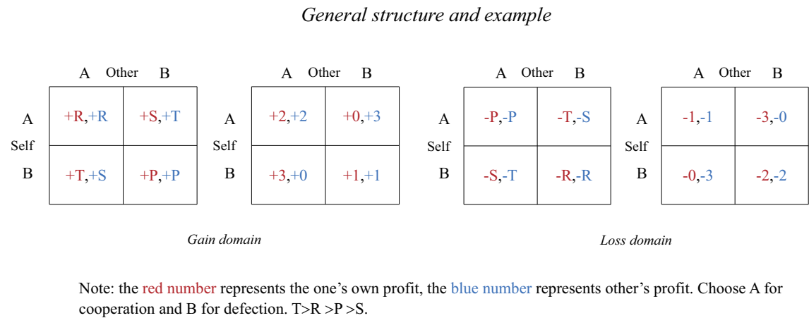
FIGURE 1: The general structure and example of the PD game according to the gain and loss domains.
