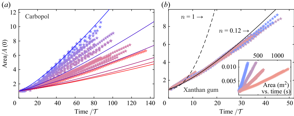
Figure 13. Plots of the area of the footprint of the film, as observed from above and scaled by the area of the pedestal for tests with (a) Carbopol and (b) Xanthan gum. The stars indicate suites of experiments with varying flux (colour from red to blue indicating increasing Q ), the lines show theoretical results for n = 0.4 and Bi = 1, 2, \dots, 6 in (a), and n = 0.12 (solid), and n = 1 (dashed) in (b) (plus Bi = 0 ). The inset in (b) shows the unscaled data; the fluxes are Q = 2.5, 5, 10 and 20 ml/min. For (a), Q = 1.25, 2.5, 5, 10, 20, 40, 60, 80, 120 and 160 ml/min.
