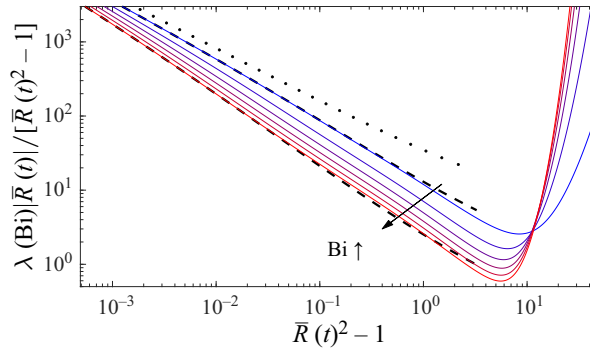
Figure 6. Time series of \lambda(Bi)|\hat{R}|/[\bar{R}(t)^2 - 1] against \bar{R}^2 - 1 for a viscoplastic film with varying Bi = 1, 2, 3, 4, 5, 6 (from blue to red), with m = 2 , n = 0.4 and \varepsilon = 10^{-4}/4 . The dashed black lines shows the prediction in (2.29) for Bi = 2 and 6 ; the dotted black line shows the prediction in (2.30) for Bi = 0 .
