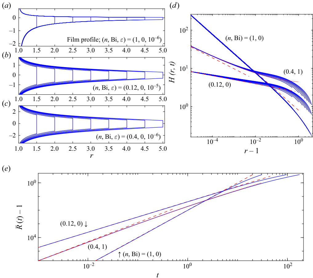
Figure 3. ( a,b,c ) Axisymmetric solutions for the values of (n, Bi, \varepsilon) indicated. Shown are film profiles at equivalent outer radii, for baths with density ratios 0.83 (panel ( a )) and \rho/\rho_b = 0.54 (panels ( b,c )). The profiles of H(r, t) are replotted on a loglog scale in ( d ) and compared with (2.21) (red dashed lines). Panel ( e ) shows time series of the outer radius \bar{R}(t) for the three solutions, with the (red) dashed lines showing (2.22). In ( d ) and ( e ) the modified early time solution (2.23) for Bi = 1 is shown by the (red) dotted lines.
