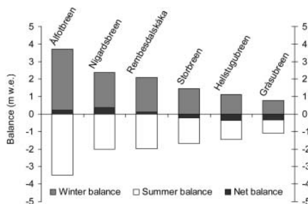
Fig. 4. Mean winter, summer and net balance for Ålfotbreen, Nigardsbreen, Rembesdalskåka, Storbreen, Hellstugubreen and Gråsubreen for the period 1963–2003.
