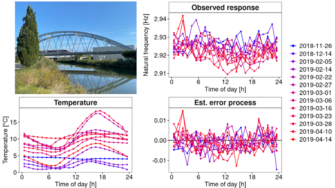
Figure 1. KW51 Bridge from the south side in September 2024 (top-left). The natural frequency of mode 6 for some selected days before the retrofitting started (top-right) and the corresponding steel temperature curves (bottom-left). If a simple piecewise linear model is used for temperature adjustment, the error profiles (bottom-right) are obtained.
