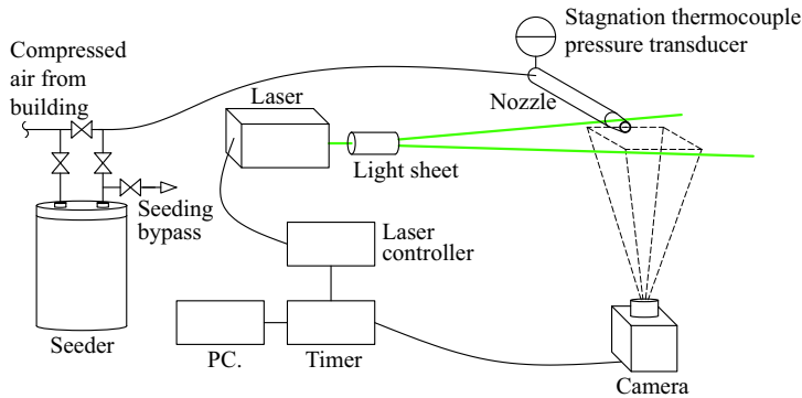
Figure 2. Schematic of free jet PIV experimental set-up.
