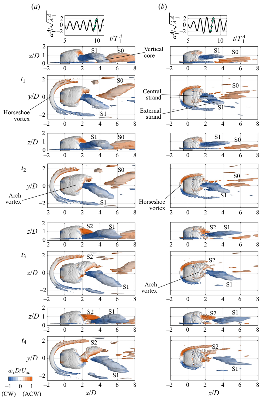
Figure 7. Isosurfaces of \lambda_2 D^2 / U_\infty^2 = -0.05 coloured by the streamwise vorticity \omega_x D / U_\infty for the flow reconstructed with the first antisymmetric mode pair at four instants indicated by the circles at the top of the figure. Here (a) \delta/D = 0.2 and (b) \delta/D = 0.8 ; T_1^A denotes the period corresponding to the dominant frequency identified for the first antisymmetric mode.
