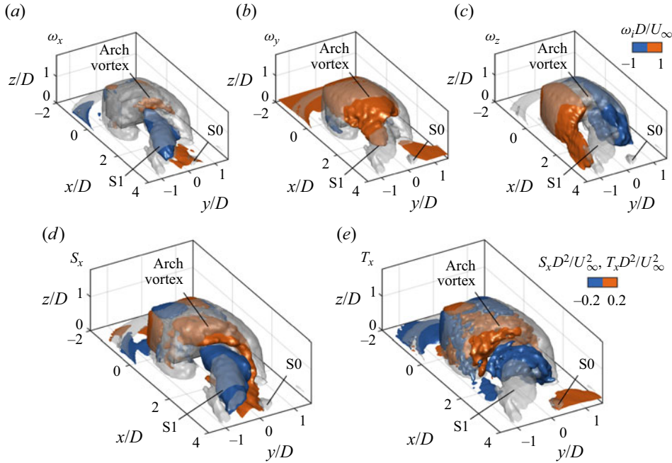
Figure 9. Isosurfaces of vorticity components and vorticity transport terms for the reconstructed flow field at instant t_1 of figure 7, for \delta/D = 0.2 . (a–c) Streamwise ( \omega_x D/U_\infty ), transverse ( \omega_y D/U_\infty ) and vertical ( \omega_z D/U_\infty ) vorticity components; (d,e) streamwise stretching ( S_x D^2/U_\infty^2 ) and tilting ( T_x D^2/U_\infty^2 ) terms. Positive values of S_x and T_x denote the generation of positive (ACW) \omega_x , and negative values correspond to negative (CW) \omega_x . The semitransparent grey isosurfaces indicate \lambda_2 D^2/U_\infty^2 = -0.05 , for reference.
