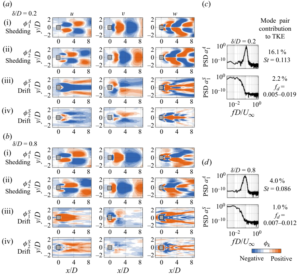
Figure 6. Contours of the spatial SPOD modes \phi_k in x - y planes at z/D = 0.5 (midheight), for the first antisymmetric and symmetric mode pairs for (a) \delta/D = 0.2 and (b) \delta/D = 0.8 . The PSD of the temporal coefficients of the first antisymmetric and symmetric modes are presented in (c,d), respectively.
