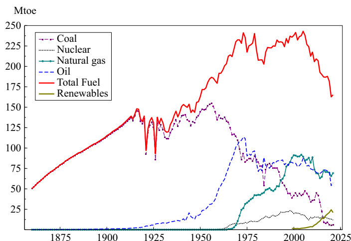
Figure 1. UK total energy use, calculated as the sum of coal, oil, natural gas, nuclear and other non-GHG, all in Mtoe.
