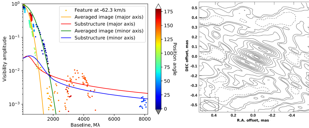
Figure 1. Left panel. Dots: relative visibility amplitude vs. baseline length for the brightest maser spot at V_{\text{LSR}} = -62.3 km/s. Lines: theoretical visibility curves for diffractive image and refractive noise. Right panel. Image of the spot at -62.3 km/s obtained with RadioAstron. The peak brightness is 2100 Jy/beam and the contours are plotted at -1 , 1 , 2 , 5 , 10 , 20 , 30 , 40 , 50 , 60 , 70 , 80 , 95 , and 95\% of the peak brightness.
