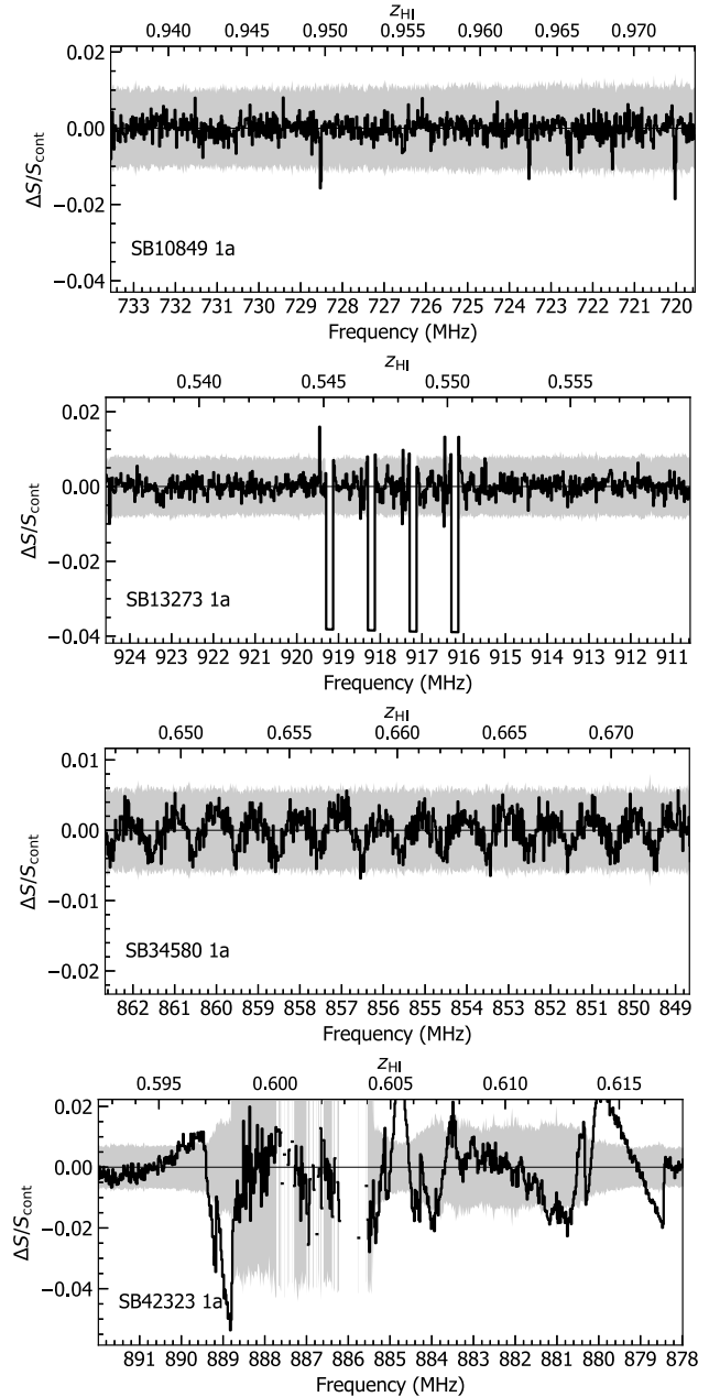
Figure 9. Examples of spectral-line artefacts seen from the Pilot data. From top to bottom, each panels presents glitches, correlator dropouts, ripples, and tropospheric ducting of RFI in spectra. The grey background shade represents five times the rms spectral-line noise.
