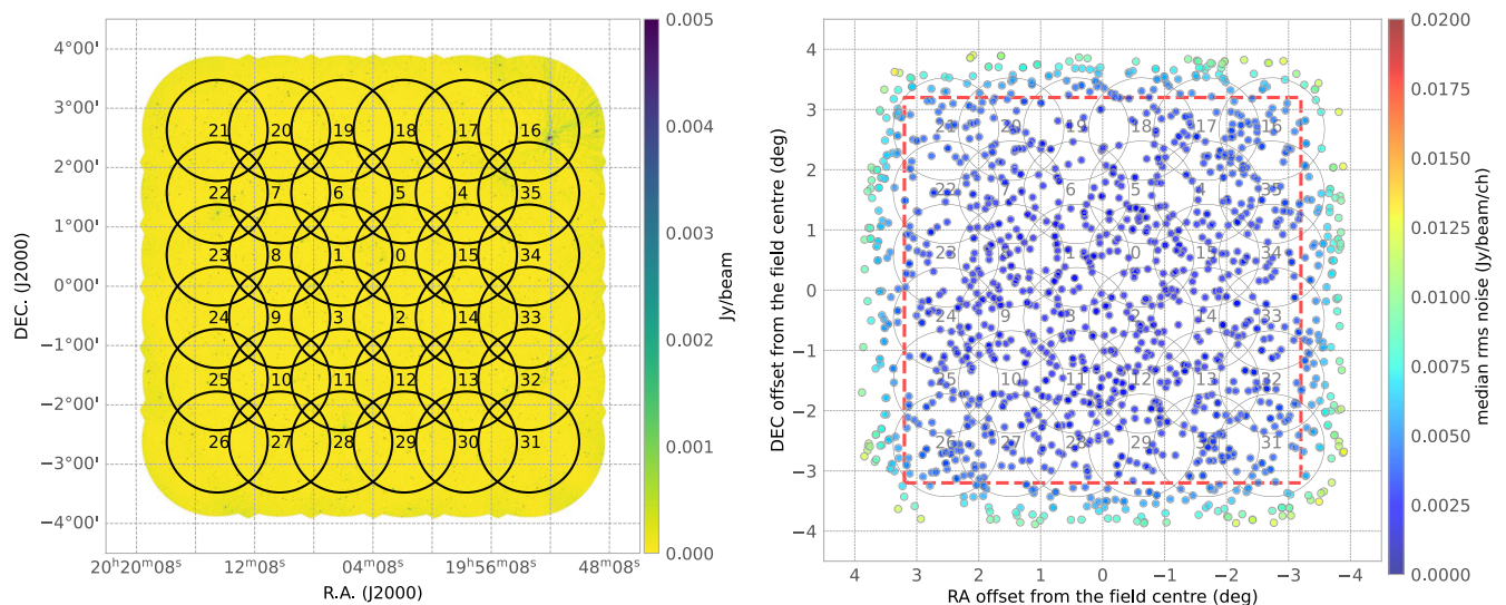
Figure 3. FLASH field of view and noise properties: (left) a FLASH continuum image showing the position of the 36 ASKAP beams in the square_6×6 footprint used to form the image, (right) measurements of spectral-line noise for extracted spectra in a 6-hour Pilot 1 observation (SBID 13293), showing that the noise is roughly uniform within the central red dashed square, covering 6.4 deg×6.4 deg on the sky (total area 40.9 deg 2 ).
