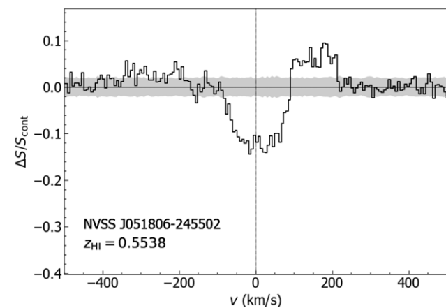
9. NVSS J051806-245502
