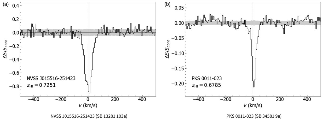
Figure 12. Two strong H I absorption lines identified in Pilot Survey Phase 1 and 2. The line profiles of all the detections are added in Appendix D. The grey shaded region in this figure and the figures in Appendix D represents 1\sigma level of the rms spectral-line noise.
