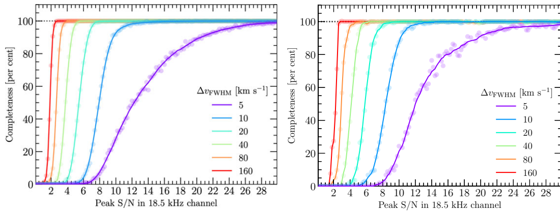
Figure 15. The completeness fractions plotted as a function of the peak signal-to-noise ratio for data from a good-quality observation (SB 34917). The colours represent a set of lines of different FWHMs, as indicated in the legend. The linefinder detection limit is set at \ln(B) > 20 for the left-hand plot, and at \ln(B) > 30 for the right-hand plot. Further details are provided in Section 8.6.
