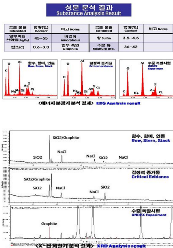
Figure 4. JIG's EDS and XRD
