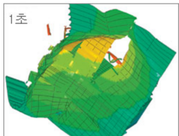
Figure 1. Cheonan's Damaged Bow and JIG's simulated damage
