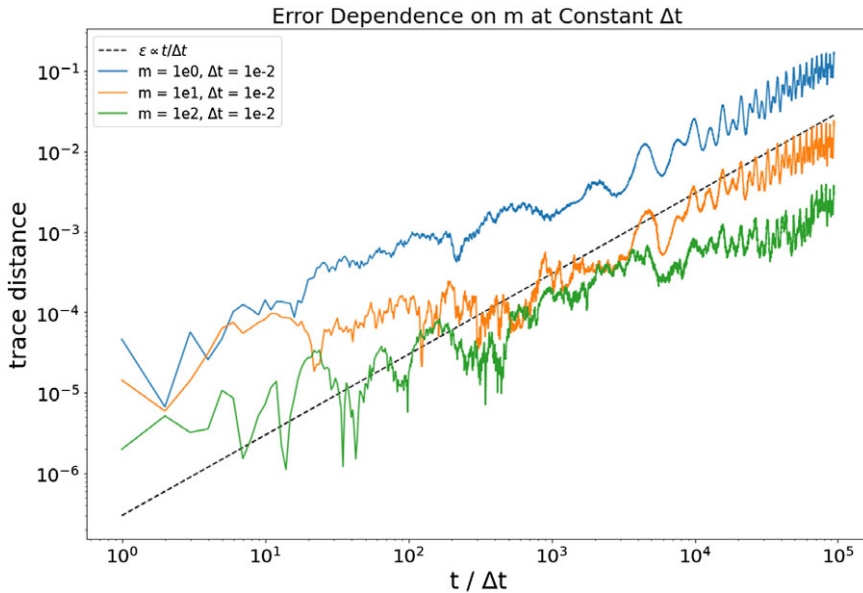
FIGURE 1. Trace distance between a deterministic solution and a stochastic, finite m ensemble of 500 independent trajectories; the error \epsilon(t/\Delta t) scales with m^{-1} and is linear in time.
