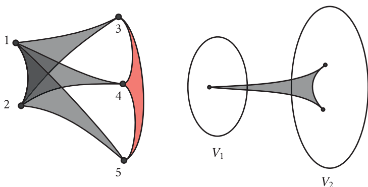
Figure 7: The 3-graph \mathbb{F}_{3,2} and the semibipartite 3-graph S_3(n) .
