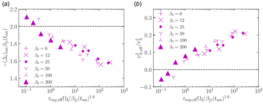
FIGURE 6. (a) Values of the firehose-instability parameter -\Delta_i \beta_{||i} at the time t_{\text{sat}} at which the square of the perturbed magnetic-field strength \delta B_f^2 / B_0^2 associated with the firehose fluctuations attains its maximum value, (\delta B_f^2 / B_0^2)_{\text{max}} , for all runs as a function of \tau_{\text{exp,eff}} \Omega_i / \beta_{||i}(t_{\text{sat}})^{1.6} . The dashed black line denotes the fluid firehose instability threshold, \Delta_i \beta_{||i} = -2 , when \beta_i \gg 1 . (b) Values of the square of the effective Alfvén speed, v_{A,\text{eff}}^2 / v_A^2 at t = t_{\text{sat}} , for all runs as a function of \tau_{\text{exp,eff}} \Omega_i / \beta_{||i}(t_{\text{min}})^{1.6} .
