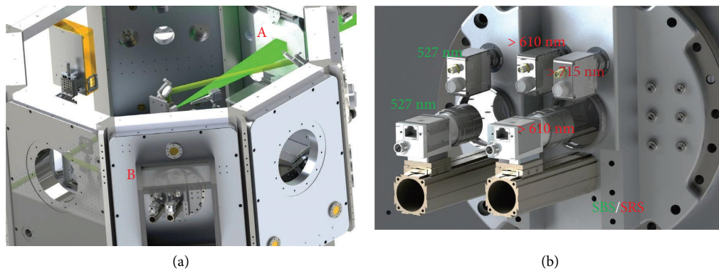
FIGURE 3: Setup of the SBS and SRS near-beam imaging diagnostics. (a) The Z-Beamlet laser enters the chamber through a hole in the PTFE screen (A). Backscattered SBS or SRS light illuminates the screen and recorded via filtered diodes and cameras in the NBI backscatter box (B). (b) Arrangement of instruments inside the NBI backscatter box.
