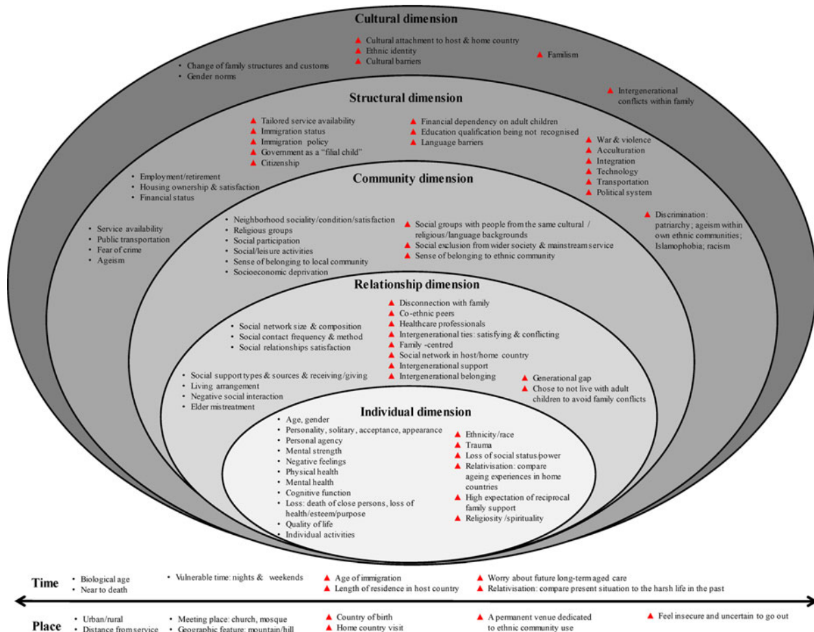
Figure 4. Mapping factors of loneliness and social isolation into a multi-dimensional socio-economical mode.
