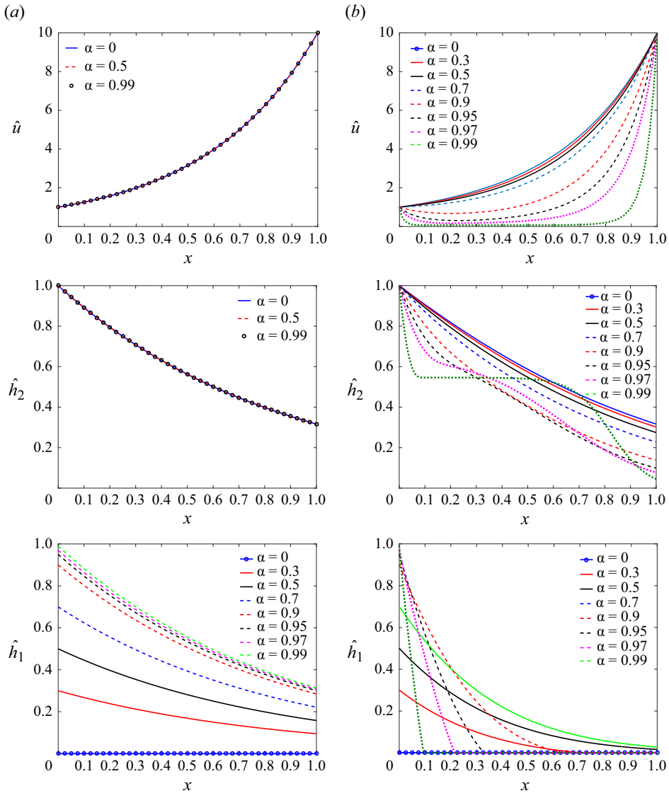
Figure 4. The effect of varying the inlet hole radius on the steady-state solution for hollow fibres without surface tension ( \Gamma=0 ) and with surface tension ( \Gamma=1 ) is shown in columns (a) and (b), respectively. In both cases the draw ratio D=10 , heat transfer coefficient C=0 , Reynolds number Re=0 and internal hole pressure P=0 .
