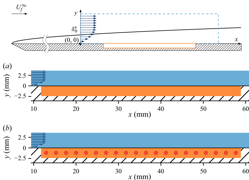
Figure 1. Wall-mounted compliant wall (orange) in a zero-pressure-gradient boundary-layer flow in water (blue). The origin of the frame of reference is positioned at the wall at the beginning of the computational domain: x and y indicate, respectively, the streamwise and wall-normal coordinates. The leading edge of the plate (i.e. the origin of the boundary layer) is positioned at x \approx -47.7 cm, for a uniform free-stream velocity U_f^\infty = 10 \text{ m s}^{-1} . The resulting Reynolds number based on the displacement thickness at the inflow ( \delta_0^* ) is Re_{\delta_0^*} = 3000 . (a) The conventional set-up from Pfister et al. (2022) with a compliant structure made by a homogeneous viscoelastic material. (b) The phononic compliant surface obtained by introducing stiffer inclusions (in red) within the homogeneous matrix and the subject of the current study.
