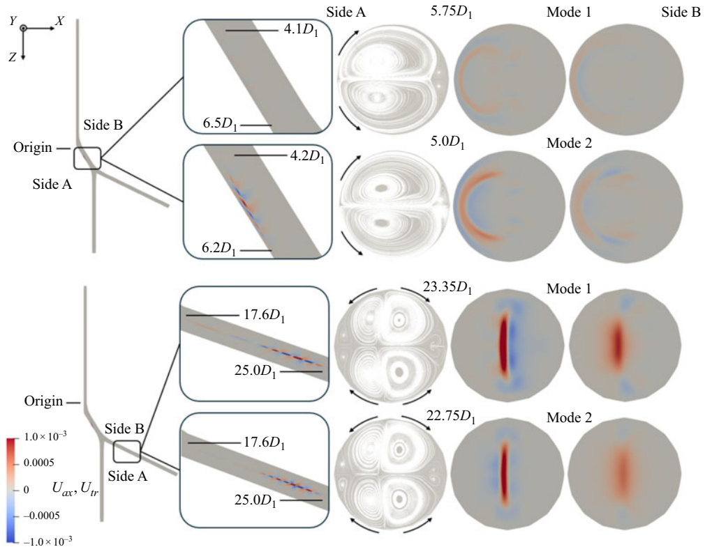
Figure 12. Leading unstable modes in the double-bifurcation inflow case, 124in . The top row of images are from the secondary pipe. The bottom row of images are from the tertiary pipe. The image on the left of each row shows the region of growth of all unstable modes in the secondary and tertiary pipes. The inset detail views show the wavelength, from top to bottom, of modes 1 and 2, respectively, as the axial component of the velocity, U_{ax} . The pipe section views show the typical base flow condition as the streamlines of the transverse component of the velocity, U_{tr} (left), the mode structure as the axial component of the velocity, U_{ax} (centre), and the mode structure as the horizontal transverse component of the velocity, U_{tr} (right). The velocity perturbations are normalised by the maximum magnitude. The left-hand side of each pipe section view (side A) pertains to the inside of the secondary or tertiary pipe (side A) of the far left image. The right-hand side of each pipe section view (side B) pertains to the outside of the secondary or tertiary pipe (side B) of the far left image. The direction of flow through the pipe sections is into the page. The curved arrows indicate the direction of the vortices. The location of each pipe section is with respect to the position along the z -axis, from the origin. The orientation of the coordinate system relates to the images on the left-hand side.
