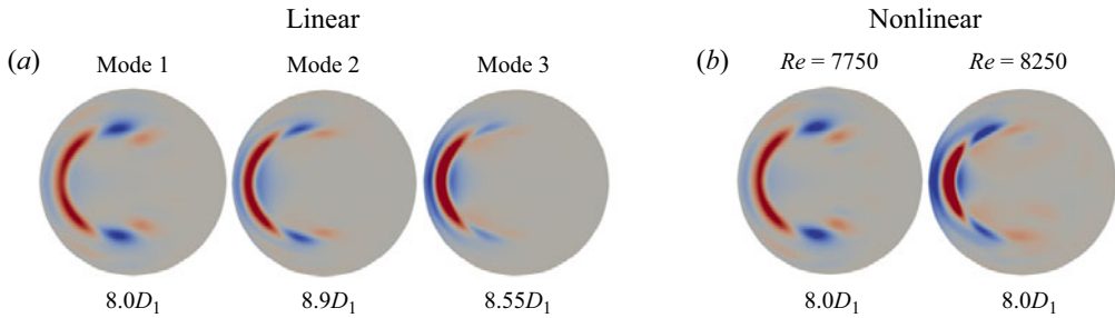
Figure 21. Comparison of linear (a) and nonlinear (b) mode structures for the single-bifurcation inflow study, 12in. The linear modes 1, 2 and 3 are identical to the images displayed in figure 11. The nonlinear mode structures from DNS are at Re = 7750 and Re = 8250 . All images are displayed as the local axial component of velocity, U_{ax} . Nonlinear mode at Re = 7750 colour range, U_{ax} \pm 10^{-4} . Nonlinear mode at Re = 8250 colour range, U_{ax} \pm 3.0 \times 10^{-4} .
