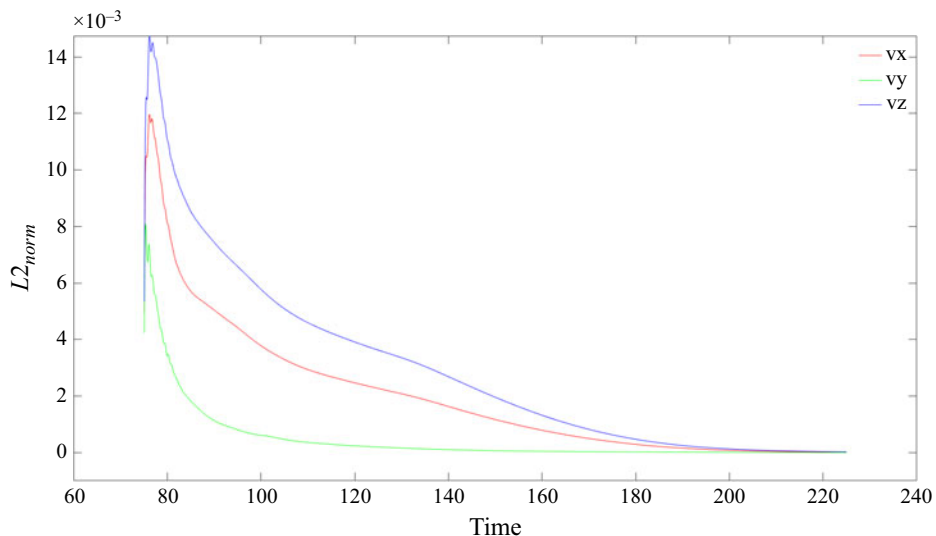
Figure 38. The SFD framework convergence test at Re = 7250 from the single-bifurcation inflow case, 12in . The three traces are outputted from the SFD algorithm plotting the global L_2 norm from each grid point after the forcing was switched on at \tau = 75 . The time history of the L_2 norm is correlated with the time history of the SFD solution (red trace) in figure 37. The SFD solution used a filter gain of 0.15 and filter width of 3.2.
