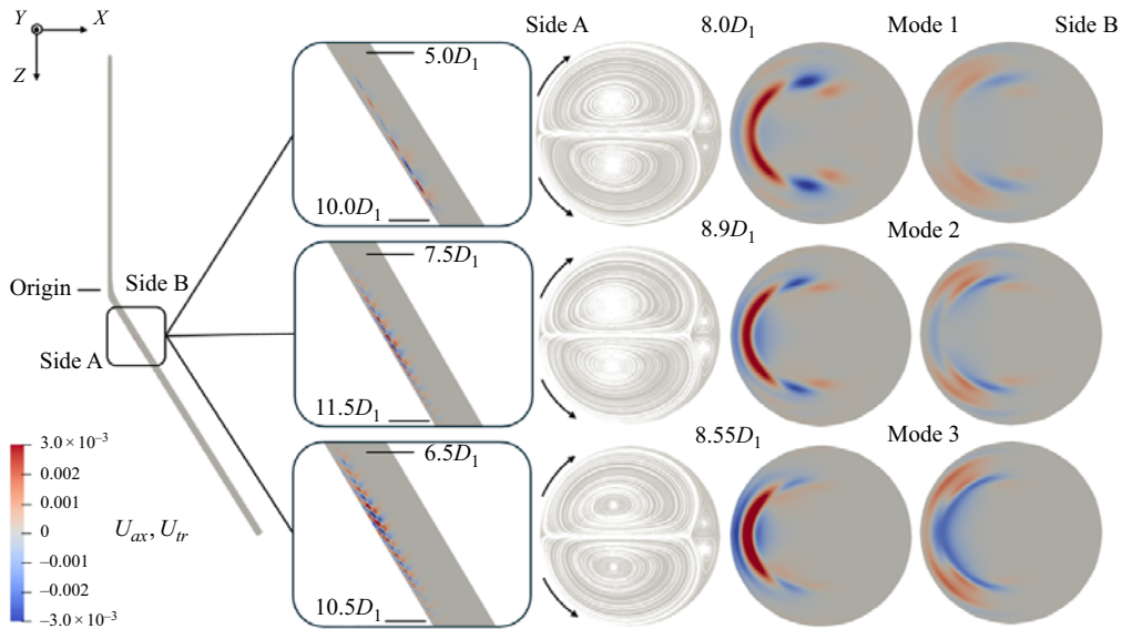
Figure 11. Leading unstable modes for the single-bifurcation inflow case, 12in. The image on the left shows the region of growth of all unstable modes in the secondary pipe. The inset detail views show the wavelength, from top to bottom, of modes 1, 2 and 3, respectively, as the axial component of the velocity, U_{ax} . The pipe section views show the typical base flow condition as the streamlines of the transverse component of the velocity, U_{tr} (left), the mode structure as the axial component of the velocity, U_{ax} (centre), and the mode structure as the horizontal transverse component of the velocity, U_{tr} (right). The velocity perturbations are normalised by the maximum magnitude. The left-hand side of each pipe section view (side A) pertains to the inside of the secondary pipe (side A) of the far left image. The right-hand side of each pipe section view (side B) pertains to the outside of the secondary pipe (side B) of the far left image. The direction of flow through the pipe sections is into the page. The curved arrows indicate the direction of the vortices. The location of each pipe section is with respect to the position along the z -axis, from the origin. The orientation of the coordinate system relates to the image on the left-hand side.
