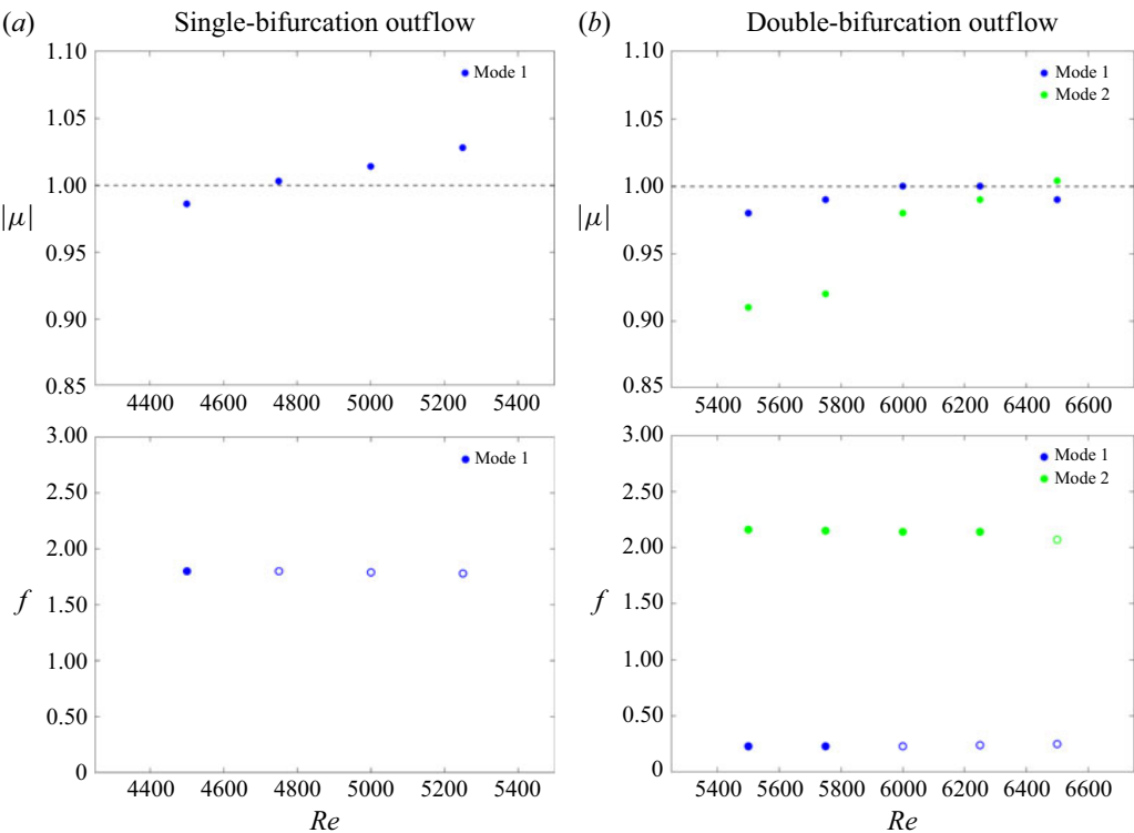
Figure 14. Multipliers, |\mu| , and frequencies, f , of the leading modes from outflow studies 12_{out} and 124_{out} plotted as a function of Re . Panel (a) shows the data from case, 12_{out} , from table 8. Panel (b) shows the data from case, 124_{out} , from table 9. The top row in each panel shows the multiplier, |\mu| , of each mode as a function of Re . The dashed line indicates where the multiplier is equal to unity. The bottom row in each panel shows the frequency, f , of each mode as a function of Re . Filled circles indicate the mode is stable. Unfilled circles indicate the mode is unstable.
