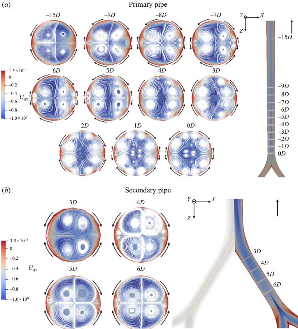
Figure 6. Double-bifurcation outflow case, 124out, base flow topology. The pipe section views display the spatially evolving stable base flow at Re = 6250 . The local axial velocity ( U_{ax} ) is overlaid by the transverse velocity ( U_{tr} ) streamlines. The left-hand side of each pipe section view pertains to the left-hand side (panel (a)) and inside (panel (b)) of the pipe from the image on the right-hand side. The direction of flow through the pipe section views is out of the page. The image on the right-hand side shows the location of each pipe section in the primary (top) and secondary (bottom) pipes. The vertical arrows indicate the direction of flow through the domain. The curved arrows indicate the direction of the vortices. The location of each pipe section is with respect to the position along the z -axis, from the origin. The orientation of the coordinate system relates to the images on the right-hand side in both panels.
