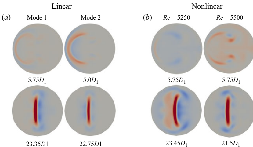
Figure 22. Comparison of linear (a) and nonlinear (b) mode structures for the double-bifurcation inflow study, 124in. The linear modes 1 and 2 are identical to the images displayed in figure 12. The nonlinear mode structures from DNS are at Re = 5250 and Re = 5500 . The images in the top row are from the secondary pipe. The images in the bottom row are from the tertiary pipe. All images are displayed as the local axial component of velocity, U_{ax} . Nonlinear mode at Re = 5250 colour range, U_{ax} \pm 10^{-2} . Nonlinear mode at Re = 5500 colour range, U_{ax} \pm 10^{-1} .
