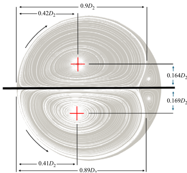
Figure 13. Comparison of the typical base flow topology present in the single- and double-bifurcation inflow cases, 12_{in} and 124_{in} . The image contrasts the size and orientation of the vortices in the single-bifurcation (bottom half) and double-bifurcation (top half) studies which trigger the linear instability after Re has exceeded the critical threshold. The red crosses indicate the location of the vortex centres. The curved arrows indicate the direction of the vortices.
