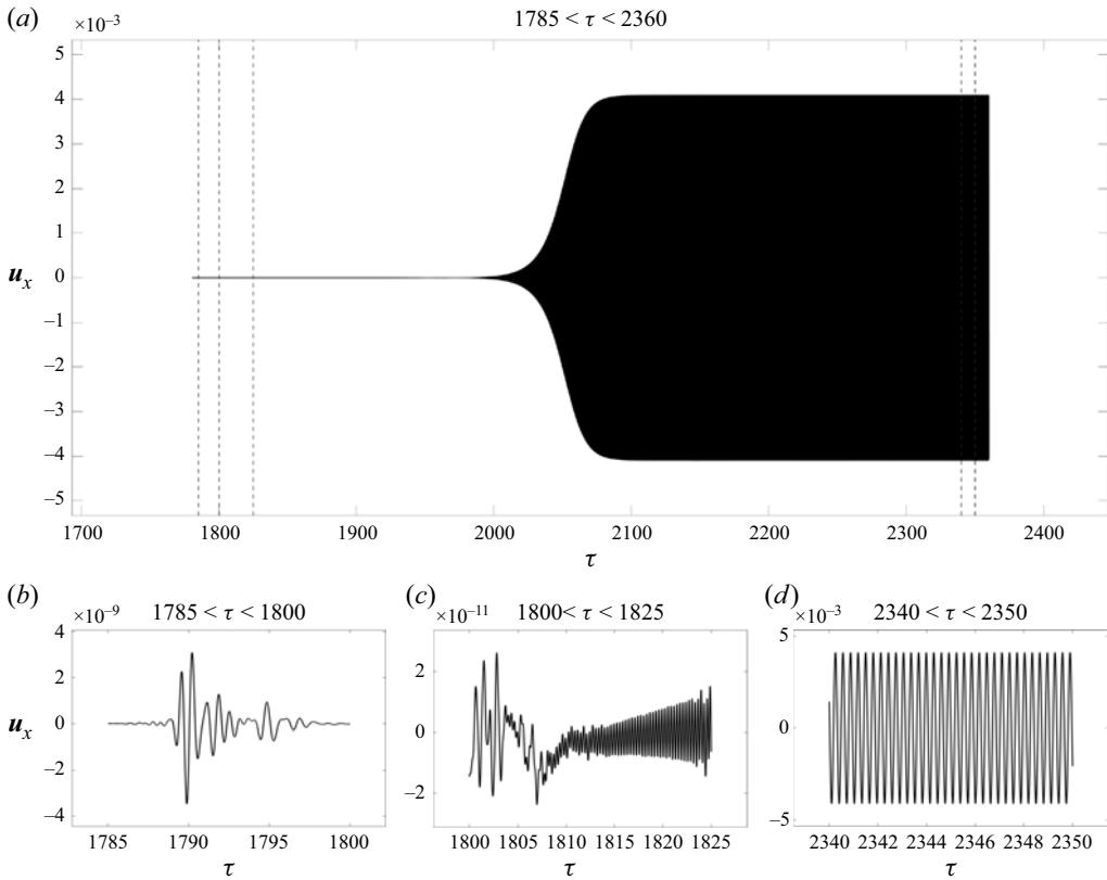
Figure 26. Velocity time series from the single-bifurcation outflow study, 12out , at Re = 4750 . The sample has been restarted from the stabilised base flow with the SFD switched off at time \tau = 1785 and run until a statistical steady state was reached. Panel (a) shows the full time series, 1785 < \tau < 2360 . Panel (b) is at time 1785 < \tau < 1800 , from the sample between the first two vertical dashed lines in panel (a). Panel (c) is at time 1800 < \tau < 1825 , from the sample between the second and third vertical dashed lines in panel (a). Panel (d) is at time 2340 < \tau < 2350 , from the sample between the fourth and fifth vertical dashed lines in panel (a). The time series is the x -component of velocity from a probe point located \approx -4.0D_1 along the z -axis, from the origin, in the primary pipe.
