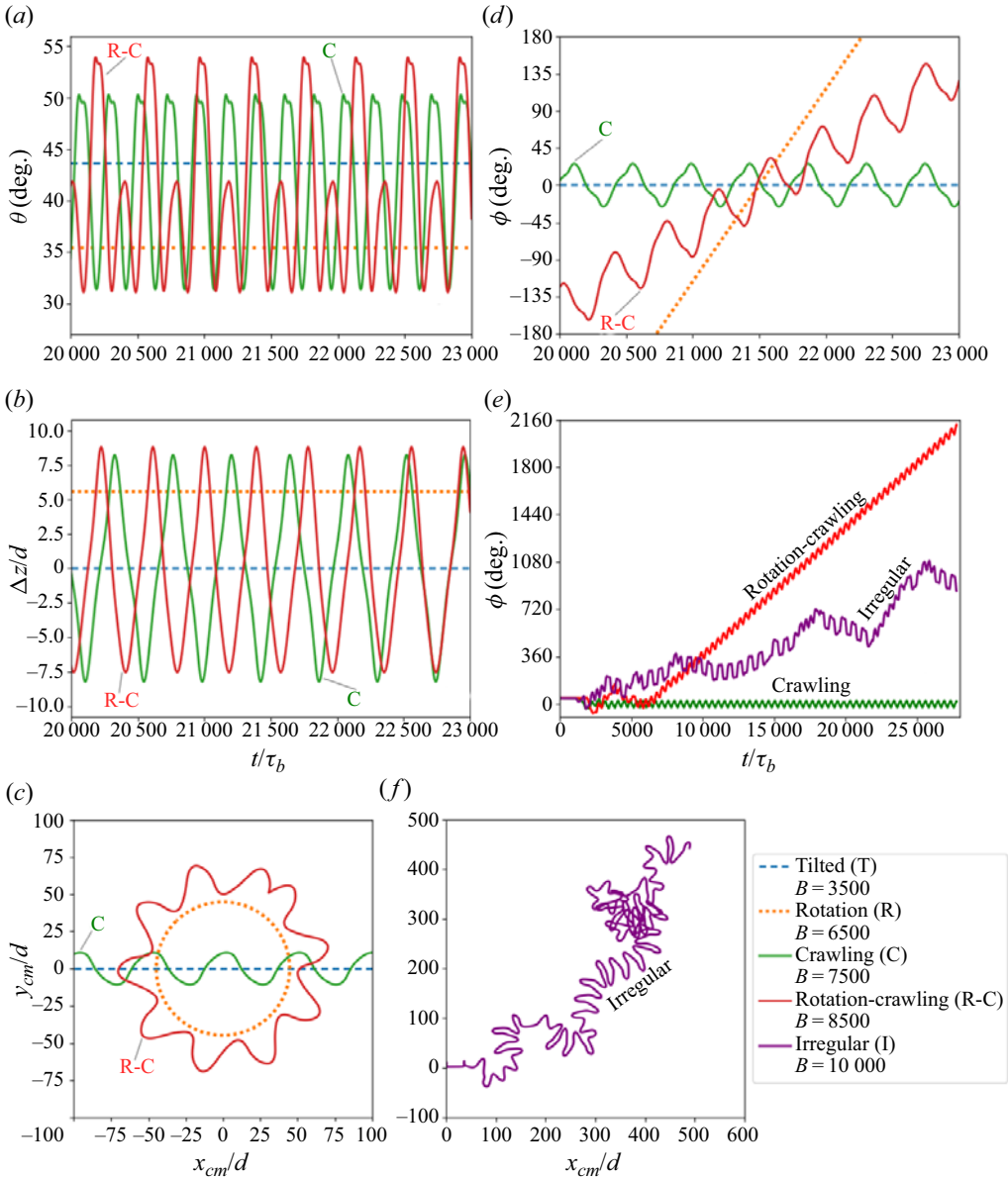
Figure 4. Basic features of the regular (a–d) and irregular (e, f) modes of fibre with N = 36 (one example of each mode). Time dependence of (a) polar angle \theta , (b) vertical coordinate \Delta z of the fibre end-to-end vector \mathbf{r}_{1N} , and (d) azimuthal angle \phi . Top view (c) of the centre-of-mass trajectory (the ranges of times are 1150\tau_b for tilted, 1545\tau_b for rotation, 1800\tau_b for crawling and 3700\tau_b for rotation-crawling modes). Evolution of an irregular mode: (e) azimuthal angle \phi (with the results for crawling and rotation-crawling modes shown for comparison) and (f) top view of the centre-of-mass trajectory.
