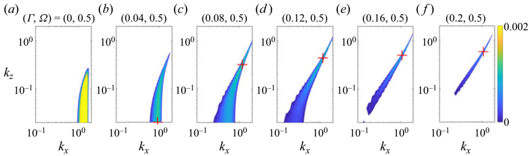
Figure 8. Same as figure 7, but now \Gamma changes gradually from 0 to 0.2, with other parameters fixed at \Omega = 0.5 , Re = 10^6 . Figure 7(f) is identical to (a). The red cross indicates where the most unstable mode is, which does not appear in (a) as the most unstable mode has k_z = 0 , and here we use log scale axes. This transition traces out the horizontal black line in figure 4. This figure further tracks the Tollmien–Schlichting branch to non-zero values of \Gamma , showing the instability found at \Gamma = 0.2 , \Omega = 0.5 is a modified Tollmien–Schlichting instability.
