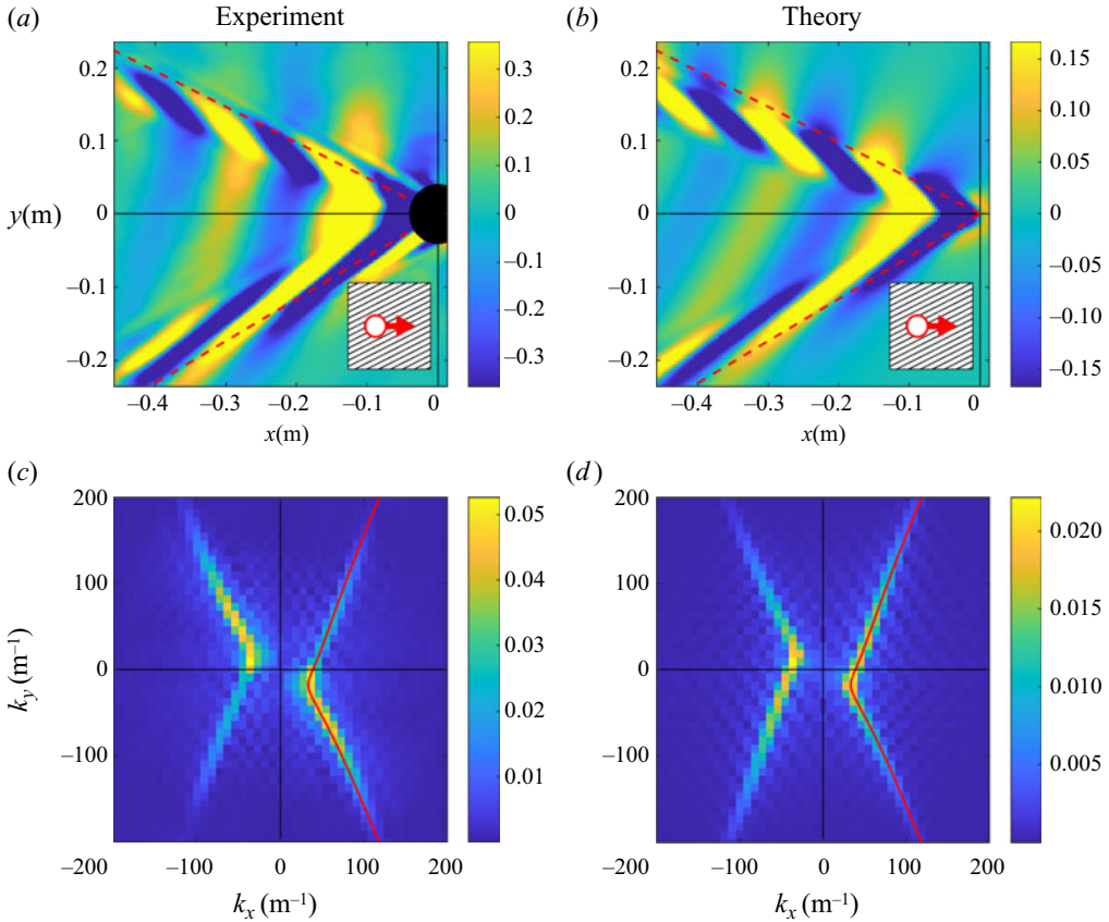
Figure 6. Surface elevation for the parameters h^- = 10 mm, h^+ = 55 mm, h_X = 12 mm, h_Y = 47.5 mm, \alpha = -62^\circ and U = 0.47 ms ^{-1} . (a) Experimental results (wave amplitude in mm); the red dashed lines indicate the maximum angle of the wake; the inset shows the layered bathymetry with the red arrow indicating the ship propagation. The colour scale is saturated to emphasize the transverse waves. (c) Fast Fourier transform of the experimental results; the red curve corresponds to the theoretical dispersion relation (2.2) and (2.3). (d) Theoretical wave amplitude obtained by Fourier transform (discretization of (A2)) and (b) the coefficients of its discrete inverse both with arbitrary amplitude.
