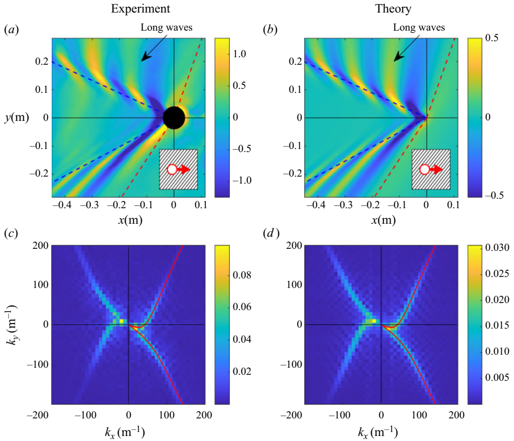
Figure 5. Surface elevation for the parameters h^- = 10 mm, h^+ = 55 mm, h_X = 12 mm, h_Y = 47.5 mm, \alpha = -39^\circ and U = 0.415 ms ^{-1} . (a) Experimental results (wave amplitude in mm); the blue and red dashed lines indicate the minimum and maximum angle of the wake; the inset shows the layered bathymetry with the red arrow indicating the ship propagation. (c) Fast Fourier transform of the experimental results; the red curve corresponds to the theoretical dispersion relation (2.2) and (2.3). (d) Theoretical wave amplitude obtained by Fourier transform (discretization of (A2)) and (b) the coefficients of its discrete inverse both with arbitrary amplitude.
