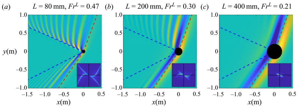
Figure 7. Theoretical wakes (and their associated Fourier transform) on the layered bathymetry with the parameters h_X = 12 mm, h_Y = 47.5 mm, \alpha = -39^\circ and a ship speed U = 0.42 ms ^{-1} . The size of the ship L varies from 80 to 400 mm (2 to 10 times the ship size in the experiments), with associated hull Froude number Fr^L from 0.47 to 0.21. The dashed curves indicate the schematic representation of the wake.
