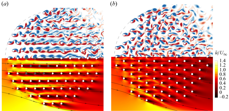
Figure 15. Cross-sectional instantaneous flow field (upper half) (at z/D=0 ) and mean field of streamwise velocity (bottom half) for (a) \theta = 0^\circ and (b) \theta = 30^\circ in an array of 109 cylinders ( G/d, D/d = (4.5, 48.6) ) in 3-D DNS. The mean flow is post-processed on a spanwise-average flow field. The colour bar (not shown) of spanwise vorticity is the same as that used in figure 14. Cylinders within TRS are marked in dark grey. With increasing \theta from 0^\circ to 30^\circ , the breakdown of TRS and channelised flow impacts relatively fewer cylinders in a large array relative to that in the smaller array in figure 14.
