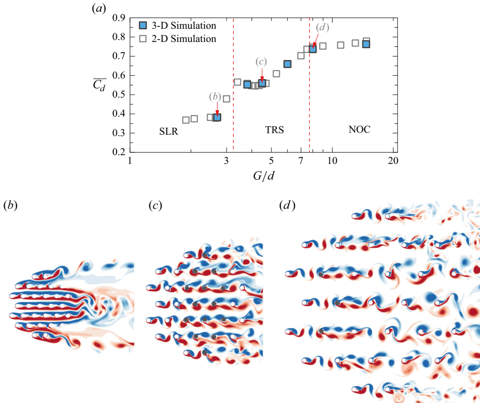
Figure 12. Demonstration of the critical role of element-scale flow structures in determining the average element drag coefficient in both 3-D and 2-D DNS. (a) Variation of \overline{C_d} with G/d for arrays with N = 31 . Dashed lines represent the range of G/d where SLR, TRS or NOC become dominant. (b–d) Cross-sectional instantaneous flow fields of N = 31 for critical gap ratios ( G/d = 2.7, 4.5, 8 ) at z/D = 0 in 3-D simulations marked in (a). In (c,d) cylinders covered by TRS are marked in dark grey. Despite the general increasing trend of \overline{C_d} , values of \overline{C_d} are controlled by the characteristic flow structures and its variation with G/d .
