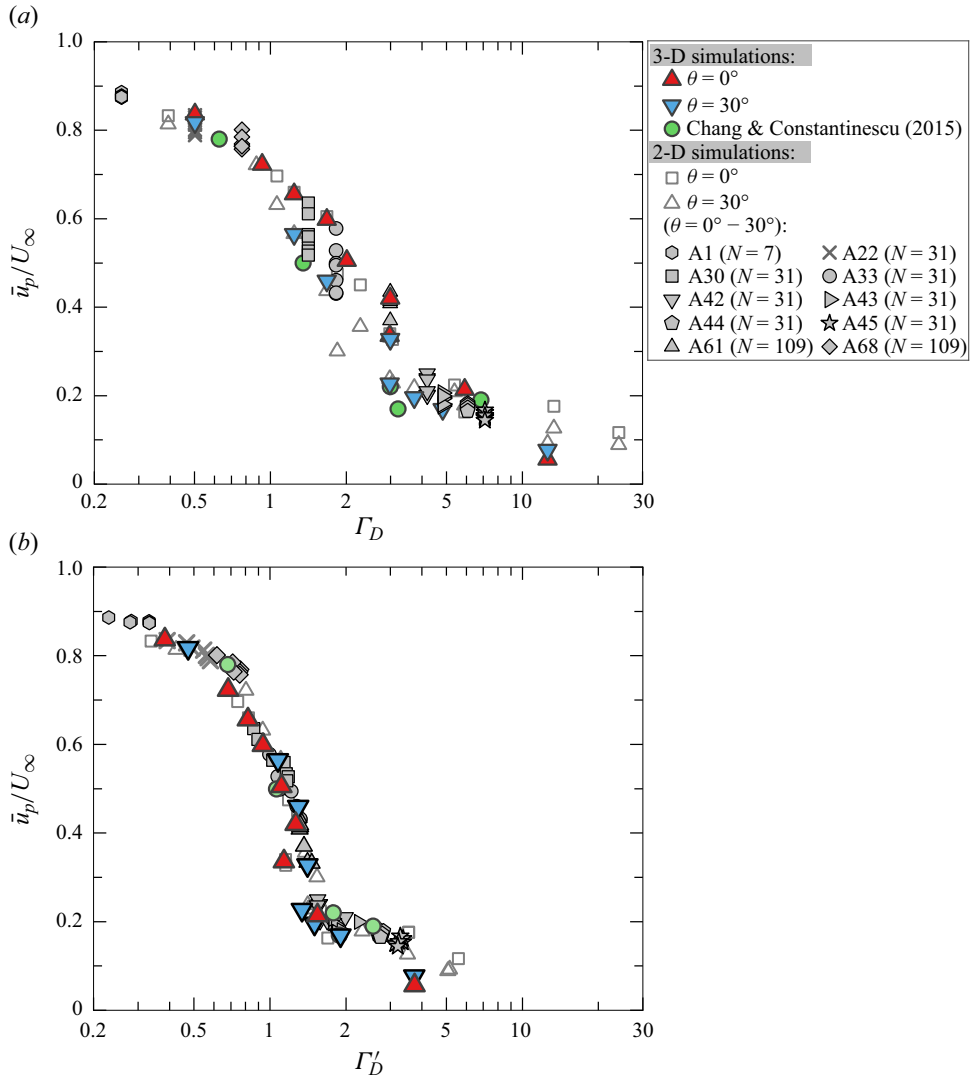
Figure 19. The relationship between the bleeding velocity \bar{u}_p/U_\infty and flow blockage parameters. Here \overline{C_d} = 1 and direct measurement of \overline{C_d} are used in (a) \Gamma_D and (b) \Gamma'_D . The filled grey symbols represent the cases varying \theta from 0^\circ to 30^\circ with an interval of 5^\circ (see table 4 in Appendix B). The data points are scattered in (a) but collapse well in (b), demonstrating that \Gamma'_D controls the bulk bleeding flow.
