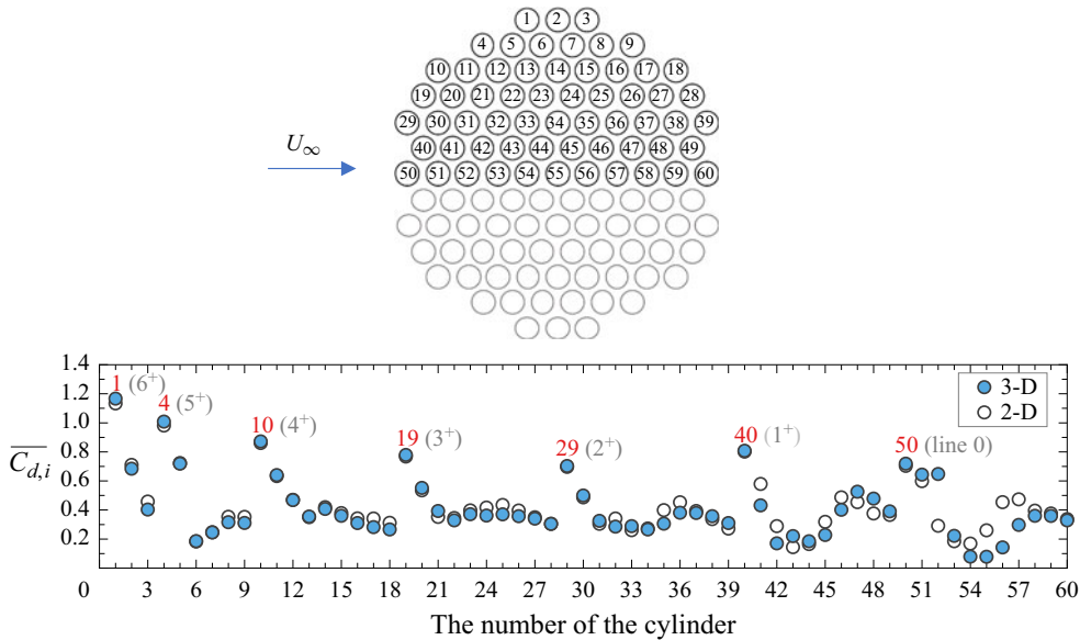
Figure 11. Distribution of drag coefficient of cylinders within an array of cylinders with N = 109 , G/d = 4.5 in both 3-D and 2-D DNS. The cross-sectional instantaneous flow field for this case is shown in figure 9(c). The distributions of \overline{C_{d,i}} along the line of cylinders within the array in both 3-D and 2-D simulations are similar to that of the single line of cylinders shown in figure 8(c), especially in the middle of the array, suggesting the applicability of using 2-D DNS in characterising the element drag.
