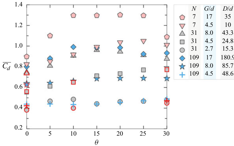
Figure 18. The strong, nonlinear variation of \overline{C_d} with \theta across the range of arrays, demonstrating that the \overline{C_d} value is not only related to the array geometry but also depends on the orientation of the array. The symbols with red and black edges represent 3-D and 2-D cases, respectively.
