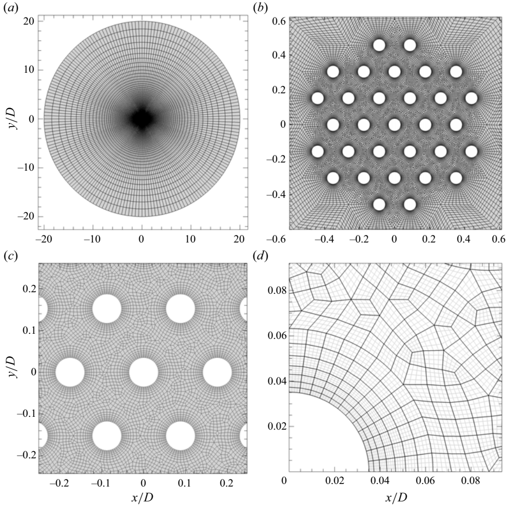
Figure 3. Mesh topology for an array of cylinders with N=31 . (a) Global view of entire computational domain; (b) close-up view of h -type mesh distribution for the cylinder array; (c) close-up view of detailed h -type mesh distribution around seven cylinders around the array centre; (d) close-up view of a hp -refined mesh around the central cylinder for which the h -type element is in black and the p -type expanded element is in grey. The overall mesh resolution is defined by both the distribution of the h -type meshes and the expansion order N_p ( =5 ) for the p -type refinement.
