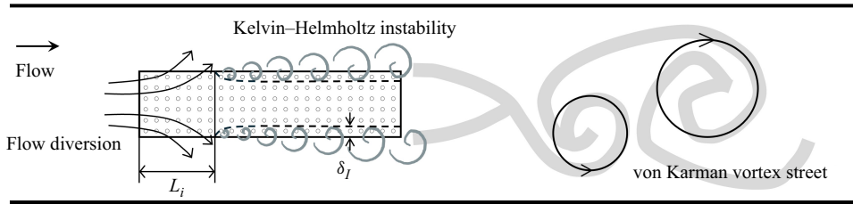
Figure 1. Top view of an emergent vegetation patch within a channel, illustrating the flow structures formed inside and in the wake of the patch. At the leading edge of the patch, the flow decelerates and is diverted laterally out of the patch over the interior adjustment length L_i . Shear layers form along each flow-parallel edge, which produce vortices by KH instability. These vortices, and the associated enhanced momentum exchange (Reynolds stress), penetrate a distance \delta_I into the patch. A von Kármán vortex street may form in the wake of the patch.
