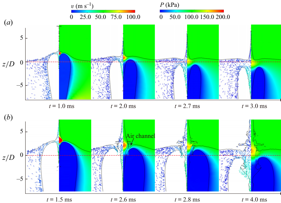
Figure 18. Flow details of the flow field evolution near the free surface. The velocity vector is on the left, and the pressure field is on the right. The black line represents the cavity wall. Panels show (a) Fr = 357.1 ; (b) Fr = 714.3 .
